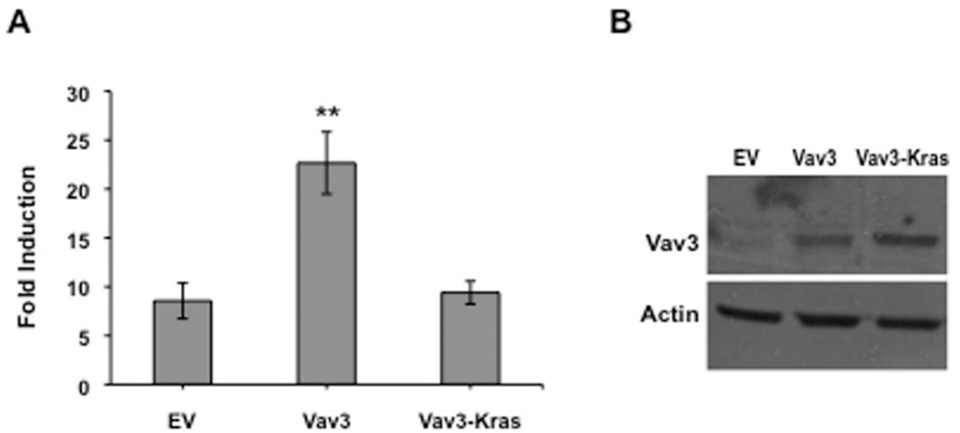
Figure 5. Membrane targeting of Vav3 eliminates Vav3 coactivation of AR
