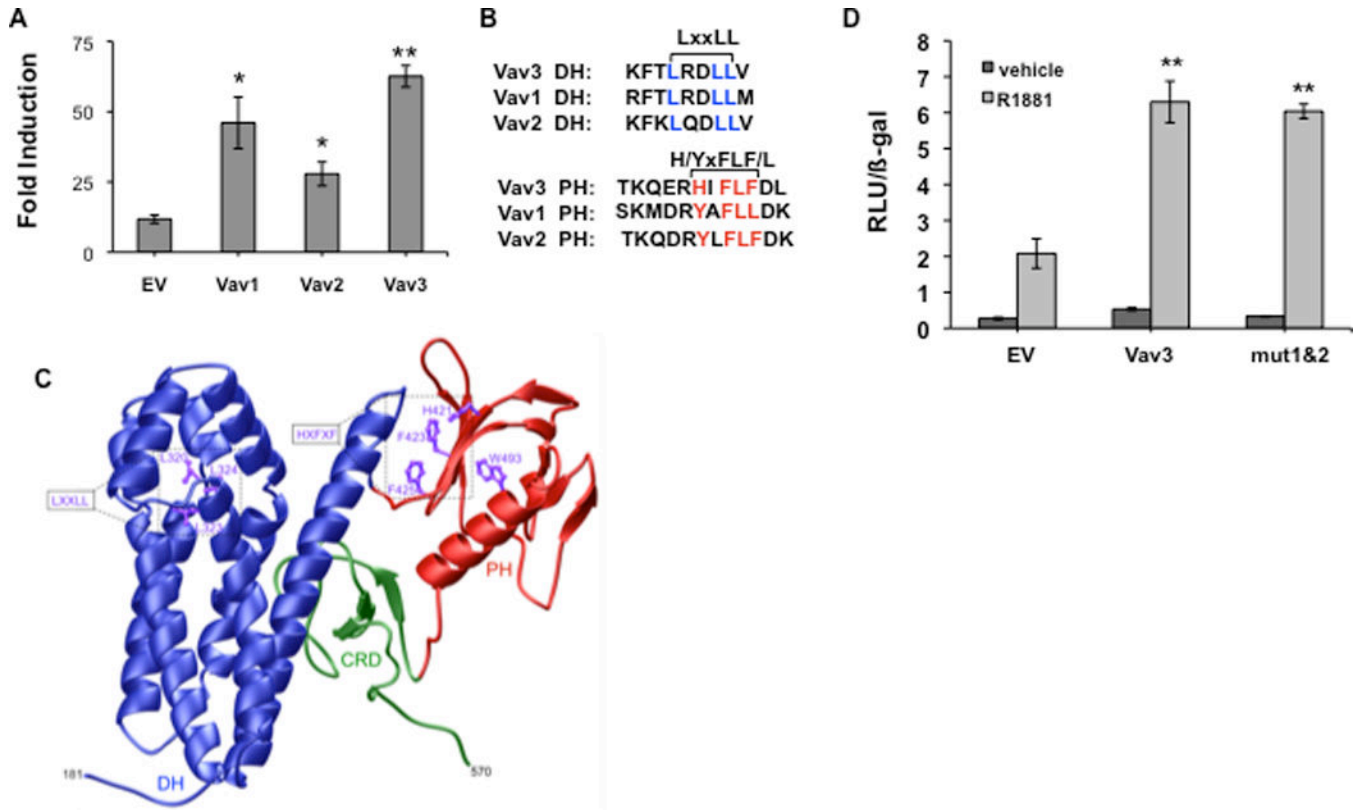
Figure 2. Vav family members enhance AR transcriptional activity but a conserved LxxLL and related motif are not required
