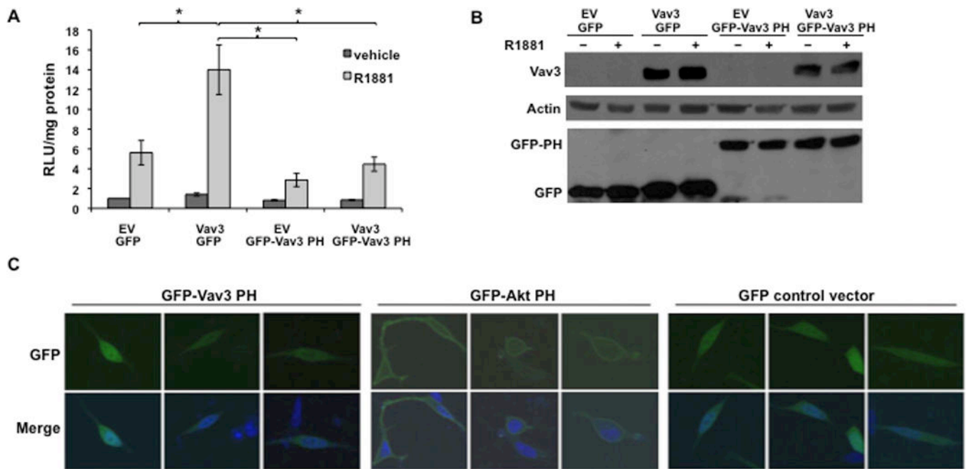
Figure 4. Vav3 PH domain alone is not sufficient to enhance AR transcriptional activity but interferes with coactivation of AR by wild type Vav3
