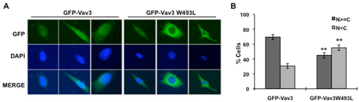
Figure 6. Vav3 PH domain confers partial Vav3 nuclear localization
