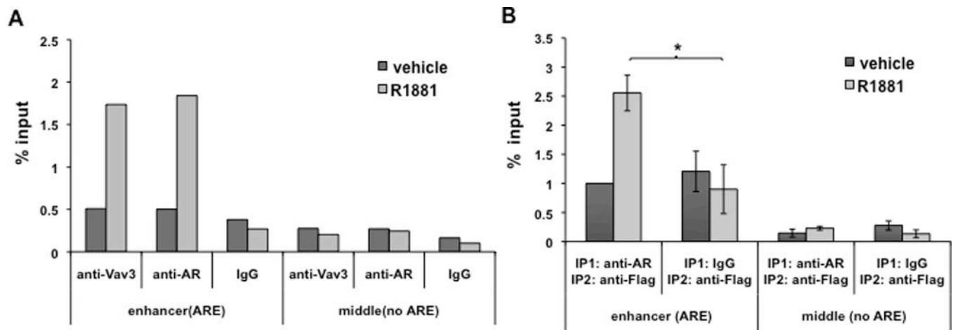
Figure 8. Vav3 and AR are recruited to the same transcriptional complexes in the PSA enhancer
