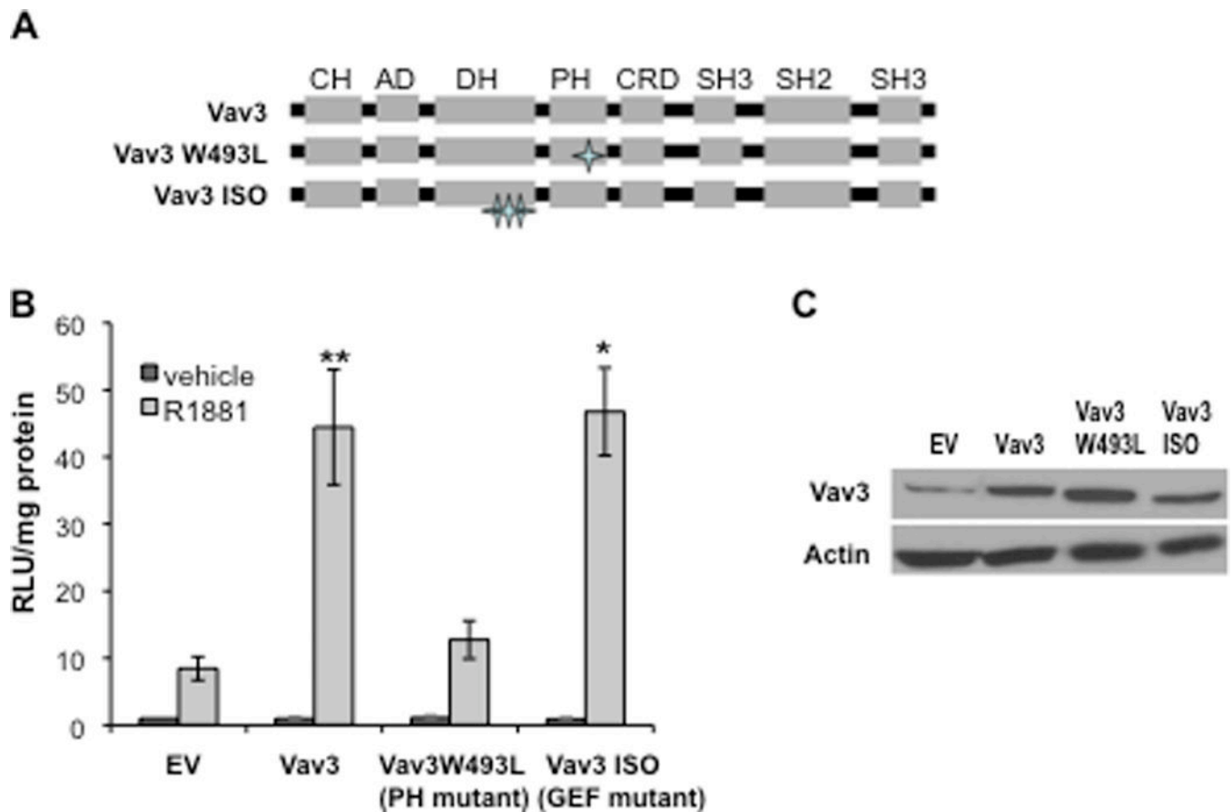
Figure 3. Vav3 increases androgen-induced AR N-C interaction in a PH dependent but GEF independent manner
