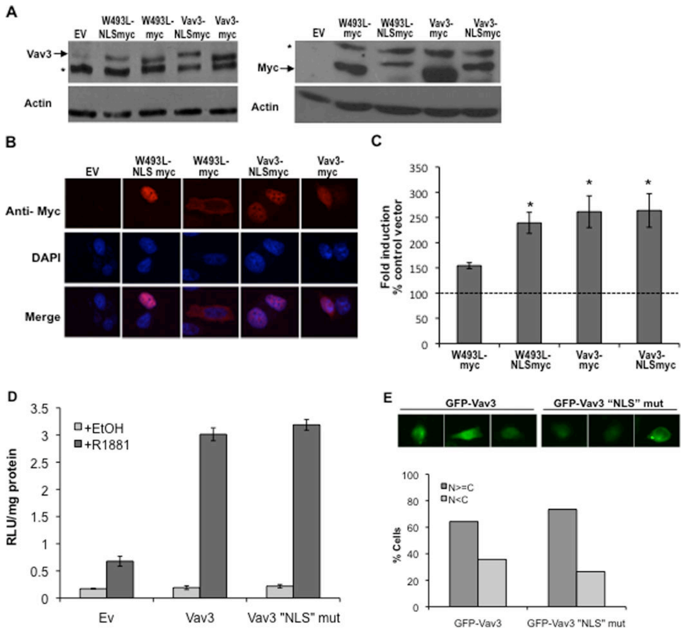
Figure 7. Nuclear targeting of Vav3 PH domain mutant (W493L) rescues AR coactivation
