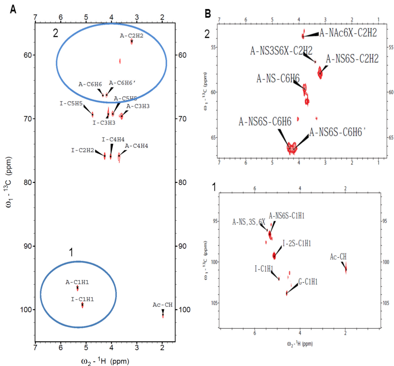
Figure 6. Two-dimensional ^1\text{H} - ^{13}\text{C} correlation spectrum (HMQC) of heparin #1. A. Entire HMQC spectrum. B. The selected regions of the spectrum. Blue circles 1 and 2 indicate anomeric region and H2/C2-H6/C6 glucosamine resonances, respectively.
