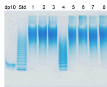
Figure 1. Polyacrylamide gel electrophoresis (PAGE) analysis on heparin samples. Lanes are: dp10, corresponding to the decasaccharide \Delta\text{UA}2\text{S}(\text{GlcNS}6\text{S}-\text{IdoA}2\text{S})_4\text{GlcNS}6\text{S} ; Std, an oligosaccharide ladder prepared by partial (30%) Hep I depolymerization of bovine lung heparin; lanes 1 to 8, correspond to heparin samples #1 to 8 (sample #4 is LMWH).
