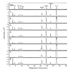
Figure 3. EIC of disaccharide analysis of 7 heparin samples and one LMWH sample by RPIP-UPLC-MS. Std shows the analysis of an equimolar mixture of 8 disaccharide standards used for peak identification and injection of different amounts afford a standard curve for quantification. Chromatograms 1–8 show the disaccharide analysis of the eight commercial heparin samples #1–#8, respectively. The peak eluting prior to 0S in each chromatogram is salt.
