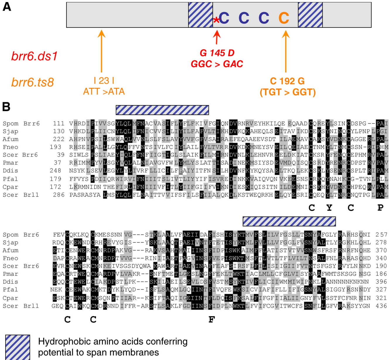
Figure 2. Brr6 structure, mutations, and homology domains. (A) A cartoon of the Brr6 protein. The brr6.ds1 and brr6.ts8 mutations are indicated in red and orange, respectively. The domains predicted to span membranes are shown with blue hatching and the highly conserved cysteines are indicated by "C." (B) Multiple sequence alignment of the conserved domains of Brr6-related proteins from the following organisms: Spom, Schizosaccharomyces pombe ; Sjap, Schizosaccharomyces japonicus ; Afum, Aspergillus fumigatus ; Scer, Saccharomyces cerevisiae ; Fneo, Filobasidiella neoformans var. neoformans ; Pmar, Perkinsus marinus ; Ddis, Dictyostelium discoideum ; Pfal, Plasmodium falciparum ; and Cpar, Cryptosporidium parvum . Amino acid sequences were aligned with the ClustalW program. Identical residues are indicated by black shading, conserved residues by gray. The single, large letters below the alignment highlight some key conserved amino acids, whereas the blocks of stripped blue shading above the alignments correspond to the hydrophobic stretches indicated in A.
