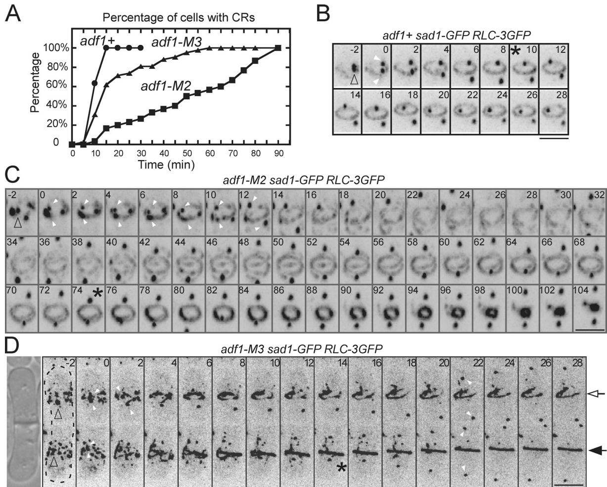
Figure 3. Contractile ring assembly in strains with cofilin mutations. (A) Time course of the accumulation of complete contractile rings in populations of wild-type ( adf1+ ), adf1-M2 , and adf1-M3 cells with the separation of SPBs at time zero. (B–D) Time-lapse series of negative-contrast fluorescence micrographs showing contractile ring assembly in cells expressing Rlc1p-3GFP and the spindle pole body (SPB) marker Sad1-GFP. Maximum intensity projections were tilted 45° to show SPBs and contractile rings and their precursors in B and C. Numbers are times in minutes after SPB separation. Empty arrowheads mark SPBs before they split and filled arrowheads mark separated SPBs. Asterisks mark the completion of contractile rings. Bars, 5 \mu m. (B) This wild-type cell assembled a complete contractile ring by time +10 min (also see Video 3). (C) This adf1-M2 cell split its SPB at time zero and condensed the nodes into clumps between time –2 to +8 min. During the following 70 min, strands containing myosin-II grew from these clumps and assembled a complete ring, which then constricted (also see Video 4). (D) Two conjoined daughter adf1-M3 cells (DIC image shown on the left) underwent the next round of cytokinesis simultaneously but differed in the time to assemble contractile rings: time +14 min for the bottom cell (filled arrow) and time +28 min for the top cell (empty arrow).
