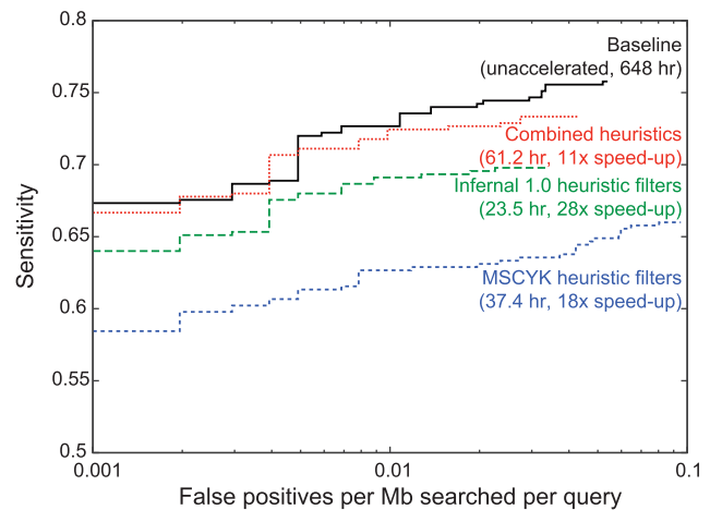
Fig. 6. ROC curves for the rmark-2 benchmark. Performance plots are shown for Infernal version 1.0, with and without the standard filtering strategy, and the new structure-based parallel filtering strategy both alone and in combination with the existing filters. All methods use default parameters for their filter cut-off values; the curve reflects only the E -value-based sort order of the final output.
