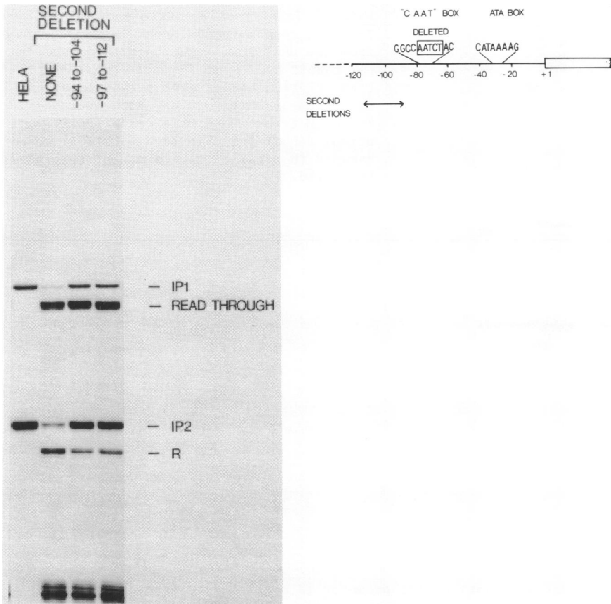
Fig. 6. The transcription efficiency of double mutant rabbit \beta -globin gene templates with lesions in the CAAT box and upstream from that site. The structures of the deletion mutants are indicated in the sequence below the figure. The second deletions were introduced at the PstI site and those analysed are indicated at the top of the figure. The signal obtained with the human \beta -globin transcripts was weak in this case and was quantitated in an over exposure of the autoradiogram. The correct rabbit transcripts were also measured relative to read-through transcripts which emanate from an upstream promoter. This approach has also been used previously (10) and gave the same results as the cotransformation approach. The terminology used is described in Fig. 3. A mock transformed HeLa cell control is included.
