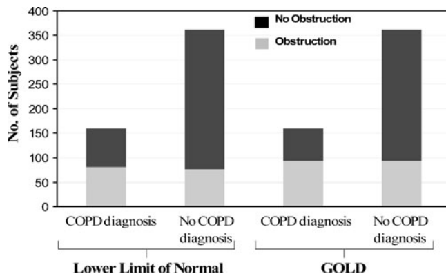
Figure 2. This figure represents patients in the cohort who had a spirometry performed. Of those who also had a diagnosis of COPD, the proportion of patients with airway obstruction as defined by the lower limit of normal and GOLD criteria is shown. Of those without a diagnosis of COPD, the proportion of patients with airway obstruction as defined by the lower limit of normal and GOLD criteria is shown.
