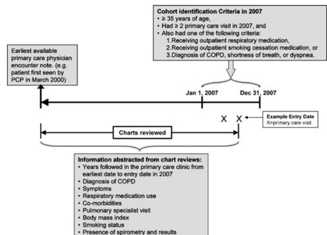
Figure 1. A diagram of the timeline of cohort inclusion and data extraction.
