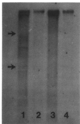
Fig. 7: Analysis of mouse and rat cell RNAs for the presence of BAM5 homologous sequences. The RNAs were isolated by a method designed to enrich for cytoplasmic RNA. Aliquots containing 10-12 ug of RNA from cultured mouse cells were untreated (lane 1) or treated with 1 ug of RNase A for 10 min. at 37 °C (lane 3). Similarly, 10-12 ug of RNA from cultured rat cells were untreated (lane 2) or RNase A treated (lane 4). The blot was probed with labeled BAM5 DNA isolated from the plasmid pMBA14. The positions of the 28S (upper arrow) and 18S (lower arrow) rRNAs in the gel are indicated.
