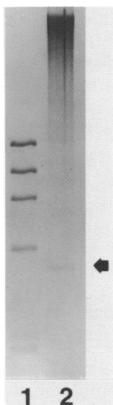
Fig. 1: Agarose gel electrophoresis of Bam HI -cleaved mouse liver DNA. 10 ug of DNA was digested to completion with Bam HI and electrophoresed into a 1.5% agarose gel (lane 2). The arrow marks the position of the BAM5 family of repetitive sequences. 1 ug of \phi X 174 RF DNA was digested with Hae III and run as size markers (lane 1). The \phi X 174 band in lane 1 just above the BAM5 band is 603 base pairs.
