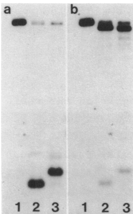
Fig. 6: Restriction mapping the 6.2 kilobase pair Bgl I repetitive fragment. The fragment (see Fig. 5, lane 5) was isolated from an agarose gel and aliquots were untreated (lane 1) or digested with Bam HI (lane 2) or Msp I (lane 3) and Southern blotted. The blot was probed with labeled BAM5 DNA isolated from the plasmid pMBA14 (a). Following autoradiography the blot was immersed in boiling water to remove the BAM5 probe and then probed with labeled 6.2 kilobase pair Bgl I fragments (b).
