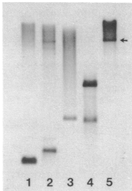
Fig. 5: Restriction mapping of total mouse DNA and detection of repetitive DNAs containing BAM5 sequences. 5 ug of mouse liver DNA was digested with Bam HI (lane 1), Msp I (lane 2), Taq I (lane 3), Hae III (lane 4) or Bgl I (lane 5) and analyzed by Southern blotting and hybridization to nick translated BAM5 DNA isolated from the plasmid pMBA14. The size of the fragment in lane 5 (arrow) was estimated to be about 6.2 kilobase pairs based upon the positions of phage lambda marker fragments (not shown).
