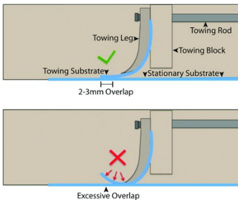
Figure 3. Culture Substrate Plating Interface. This cartoon depicts the components of the towing mechanism within each lane of the bioreactor from side view. (Top) Correct overlap of the towing and stationary culture substrates. (Bottom) Excessive overlap of the towing and stationary substrates causes the tip of the towing substrate to curl.
