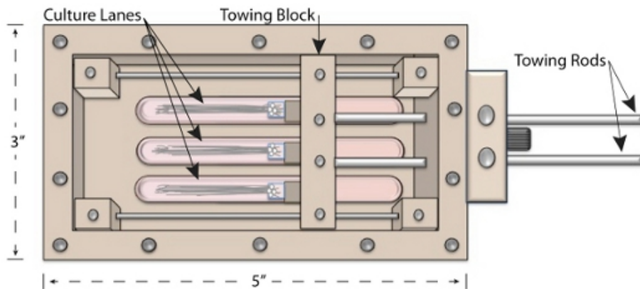
Figure 2. Bioreactor Culture Chamber. This cartoon depicts the bioreactor chamber from the top with the lid removed. The position of the towing block reflects the end stage of axon stretch growth. Stretch grown axons can be seen in bundles within the culture lanes.
