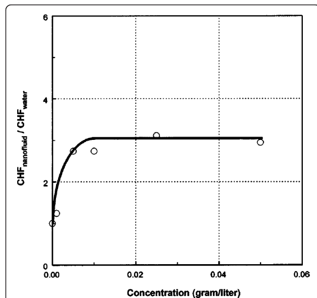
Figure 3 Graph illustrating CHF nanofluids /CHF water at different concentrations (g/l) of nanoparticles [4].
