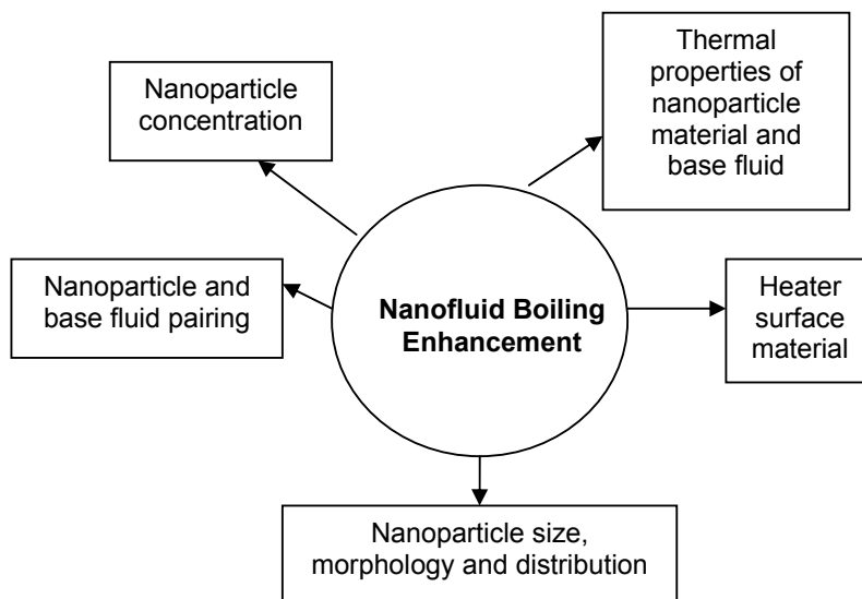
Figure 10 Factors affecting nanofluid boiling enhancement.
