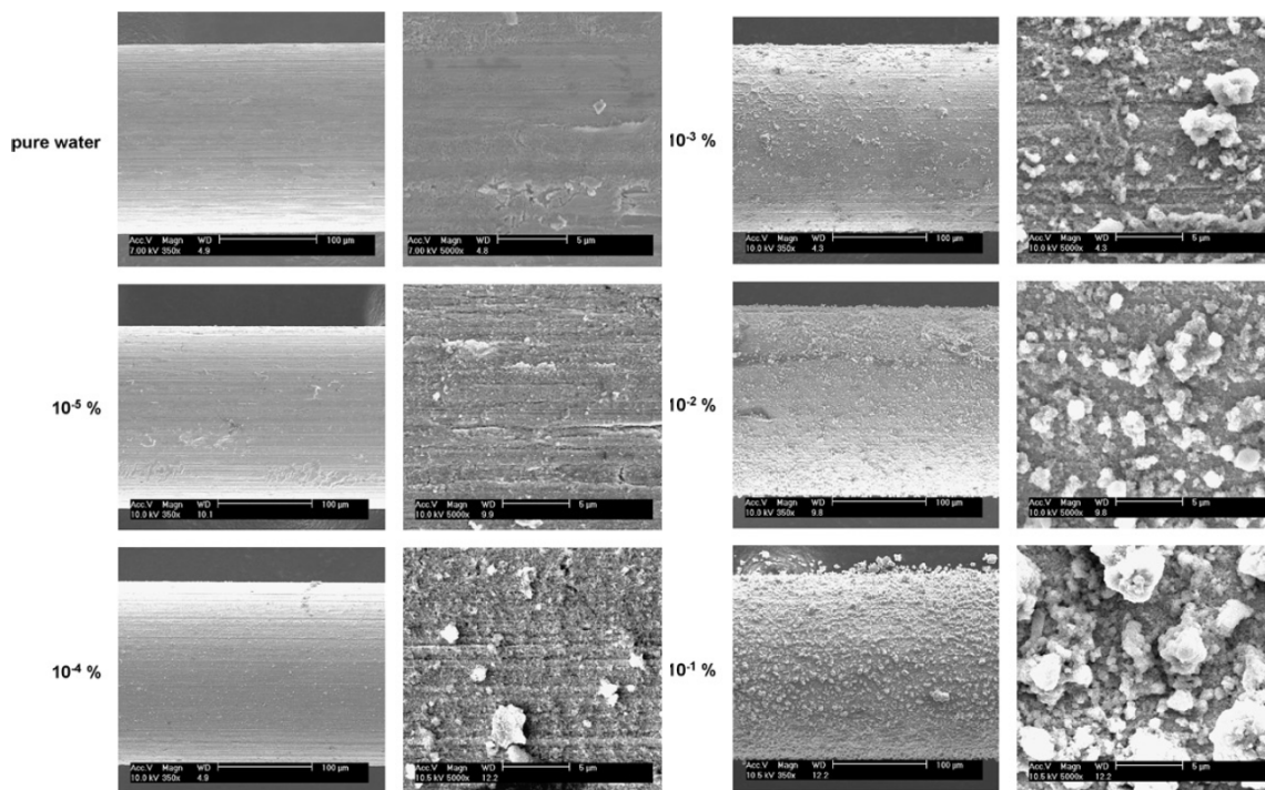
Figure 5 TiO 2 nanoparticle-coated NiCr wire after pool boiling CHF experiment of nanofluids with different particle volume concentrations [34].
