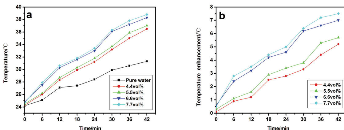
Figure 3 Photothermal properties of carbon black nanofluids. (a) Temperature as a function of time, (b) temperature enhancement as a function of time.
