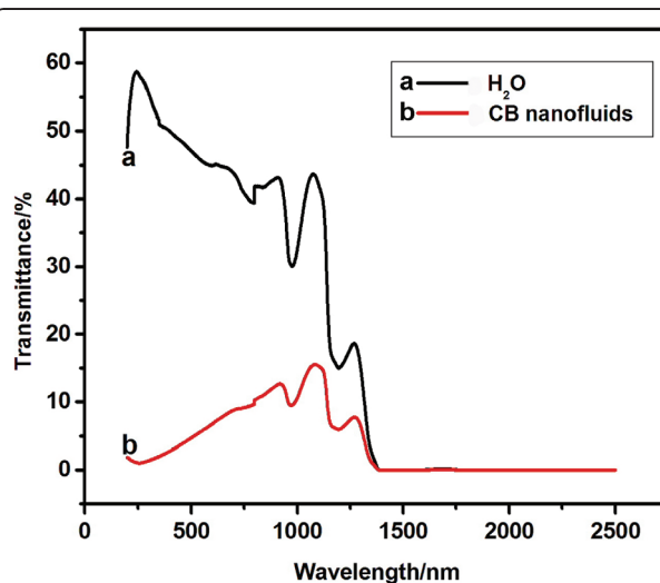
Figure 5 UV-Vis-NIR transmittance spectra. (a) Water, (b) carbon black nanofluids.
