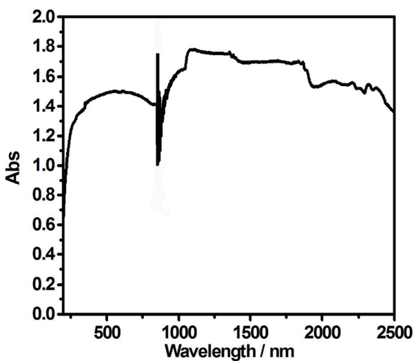
Figure 4 UV-Vis-NIR absorption spectra of carbon black powder.
