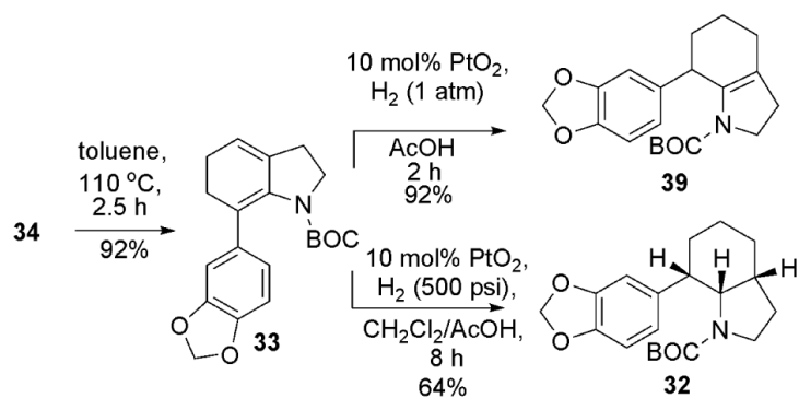
Scheme 7. Preparation of the indolizidine substructure of \gamma -lycorane ( 1 )
