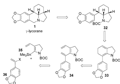
Scheme 5. Retrosynthetic analysis for the synthesis of \gamma -lycorane ( 1 )
