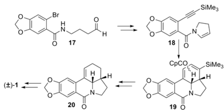
Scheme 2. Vollhardt AD \rightarrow ADC \rightarrow ADCB approach to \gamma -lycorane ( 1 )
