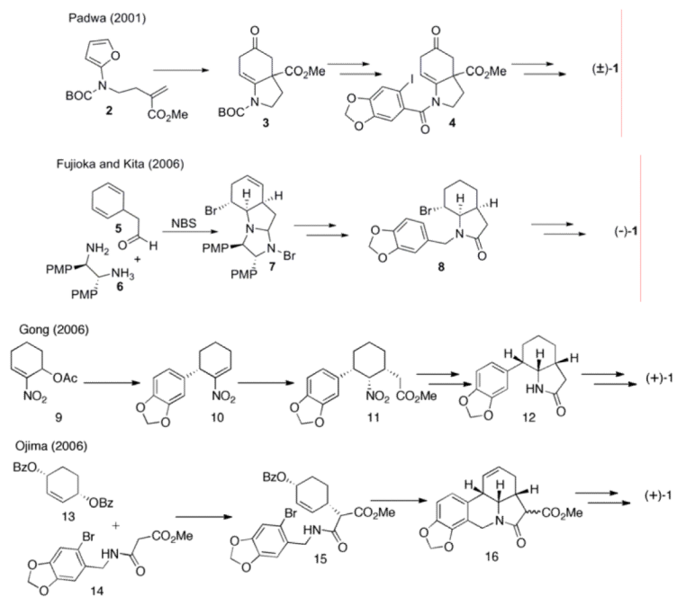
Scheme 1. CD → CDA → CDAB and AC → ACD → ACDB approaches to \gamma -lycorane ( 1 )
