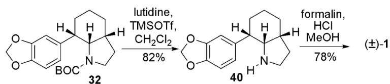
Scheme 8. Completion of the \gamma -lycorane ( 1 ) total synthesis
