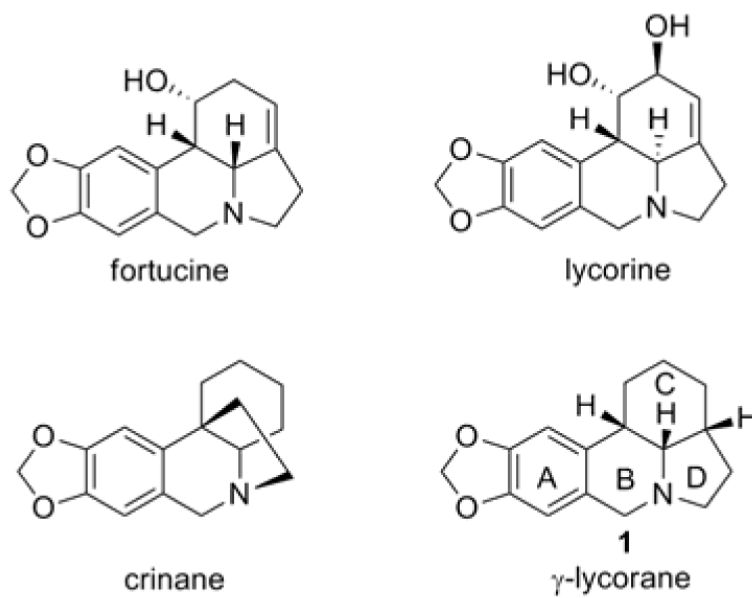
Figure 1. Selected Amaryllidaceae alkaloids
