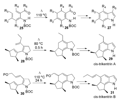
Scheme 4. Indole syntheses via trienecarbamate electrocyclizations
