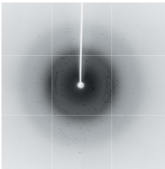
Figure 3 Diffraction image ( 1^\circ oscillation) of a NALP3 PYD crystal with a 1.7 Å resolution limit.
