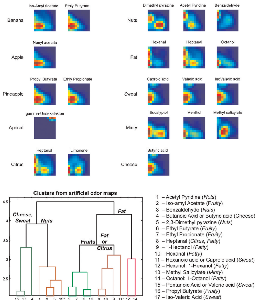
Figure 6. Artificial odor maps show how sensor responses can be linked to perceptions. Top: Chemicals associated with 10 different smell perceptions predicted from their infrared absorption spectra were organized into these maps using the chemotopic convergence model (see Figure 5a). Dendrograms (complete-linkage) revealed that artificial odor maps formed from their infrared absorption spectra formed clusters determined by organoleptic descriptors provided by human experts (from www.flavornet.org/ ). A cluster analysis of olfactory bulb activation patterns elicited by the same 17 chemicals 36 revealed qualitatively similar results (not shown). Asterisk identifies a chemical with a smell descriptor different from other members in the cluster. (Reprinted with permission from ref 94. With kind permission of Springer Science + Business Media).
