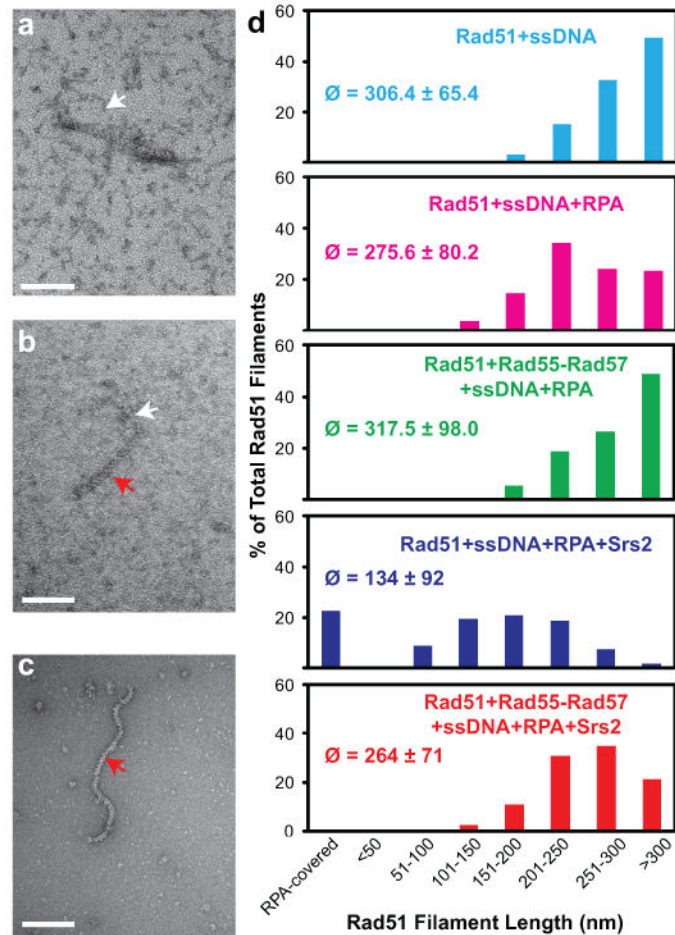
Figure 3. Rad55-Rad57 inhibit disruption of Rad51 presynaptic filaments by Srs2 a , RPA-ssDNA complex. b , Short (145 nm) Rad51-ssDNA filament. c , Long (350 nm) Rad51-ssDNA filaments d , Quantitation of electron microscopic analysis. 300-400 filaments were analyzed for each reaction condition (2.34 \mu M Rad51, 7 \mu M (nt) 600 nt ssDNA, \pm 0.43 \mu M Rad55-Rad57, \pm 0.21 \mu M RPA, \pm 0.4 \mu M Srs2), and the means ( \bar{x} ) \pm 1 sd and distributions of filament length classes are shown. Scale bars: 100 nm. White arrows indicate RPA-ssDNA complexes and red arrows Rad51 filaments.
