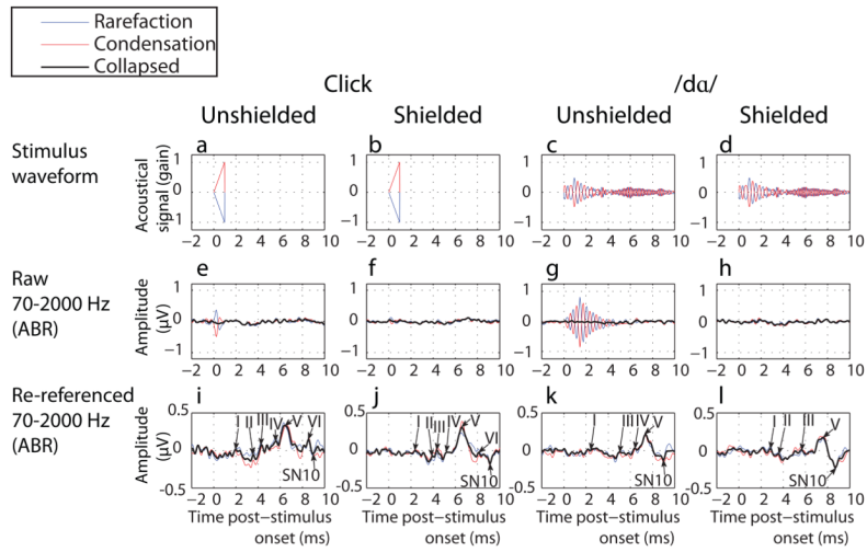
Figure 1. The stimulus waveform (a-d) used to elicit ABRs (e-l) that are plotted as a function of shielding, reference and leading phase. Please note the different scale for the referenced waveform where ABRs are visible and the large artifact eliminated. ABR peaks are labeled by Jewett-nomenclature.
