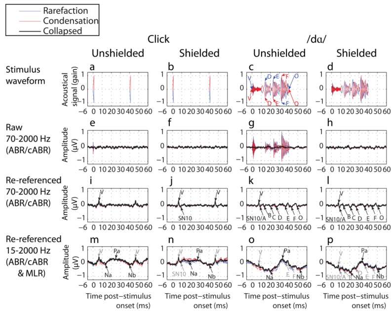
Figure 2. The stimulus waveform (a-d) used to elicit cABRs (e-l) that are plotted as a function of shielding, reference and leading phase, together with the effect of a more open filter for referenced data that yields overlapping MLRs (m-p). ABR and MLRs labels follow Jewett- and Picton-conventions; cABRs are labeled according to Skoe and Kraus (2010), as are corresponding landmarks in the stimulus waveform.
