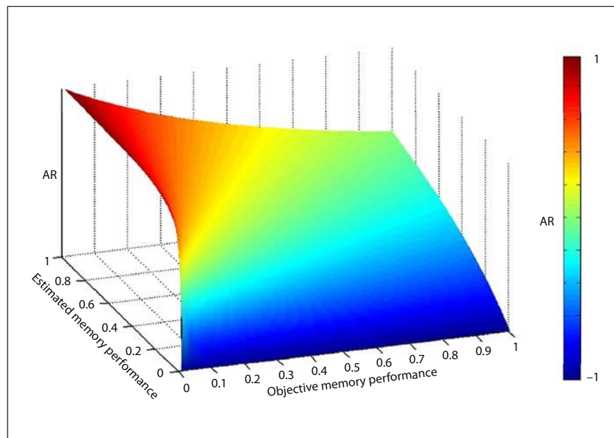
Fig. 1. Conceptual relationship between estimated and objective memory performance, described by AR equation.
