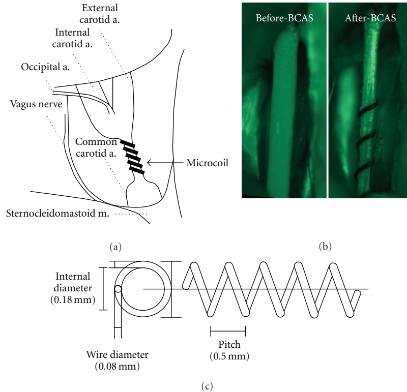
FIGURE 1: The procedure for BCAS and the microcoil. The microcoil is twined by rotating it around the CCA just proximal to the carotid bifurcation of a C57BL/6J mouse (a). Representative photographs of a FITC-perfused common carotid artery before (left) and after (right) placement of a microcoil (b). The microcoil is made from piano wire (wire diameter of 0.08 mm) with an inner diameter of 0.18 mm, pitch 0.50 mm, and total length 2.5 mm (c).
