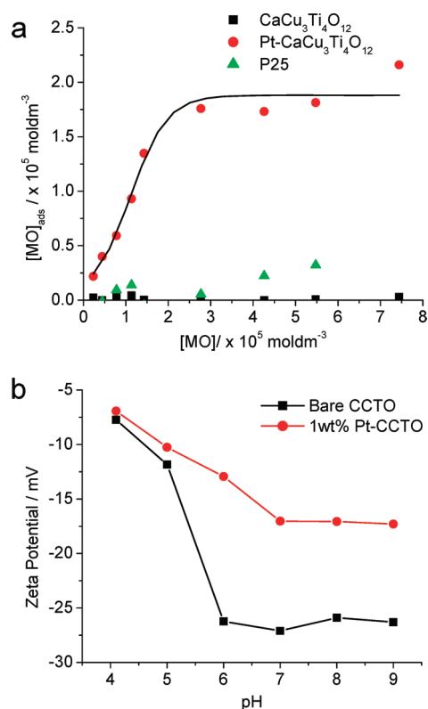
Figure 10. (a) MO adsorption isotherms of Pt-CaCu 3 Ti 4 O 12 , bare CaCu 3 Ti 4 O 12 , and TiO 2 P25. Curve is a guide for the eye. (b) Zeta potentials of CaCu 3 Ti 4 O 12 and Pt-CaCu 3 Ti 4 O 12 at pH 4–9.
