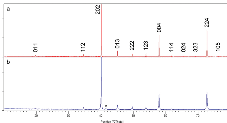
Figure 3. Powder X-ray diffraction patterns of \text{CaCu}_3\text{Ti}_4\text{O}_{12} produced via (a) ceramic and (b) sol-gel synthesis indexed to cells of Im\bar{3} , a \approx 7.39 \text{ \AA} . Asterisk denotes CuO impurity.
