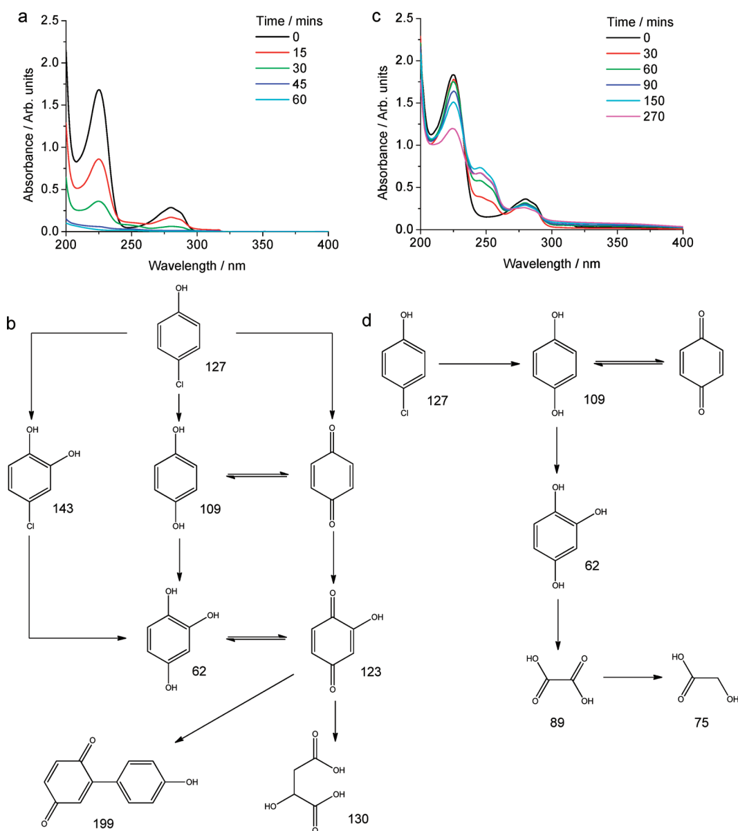
Figure 12. Spectral evolution of 4CP and photo-oxidation products (detected by MS) with UV light irradiation in the presence of 0.1 g of P25 (a,b) and 0.1 g of Pt-CaCu 3 Ti 4 O 12 (c,d).
