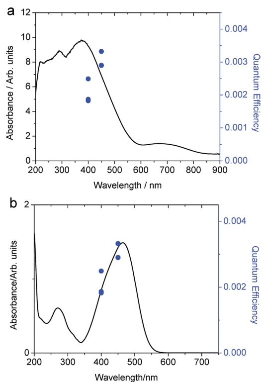
Figure 11. Quantum yields of MO oxidation over Pt-CaCu 3 Ti 4 O 12 at 400 and 450 nm (10 nm band filters) overlaid with absorption spectra of (a) CaCu 3 Ti 4 O 12 and (b) MO. Results indicate a dye-sensitized mechanism.
