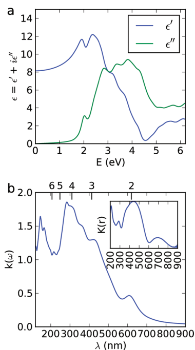
Figure 7. Calculated (a) dielectric function and (b) extinction coefficient of \text{CaCu}_3\text{Ti}_4\text{O}_{12} . The extinction coefficient is plotted against wavelength to aid comparison with experimental diffuse reflectance spectra, which is shown in the inset. The corresponding energy scale, in eV, is shown above.
