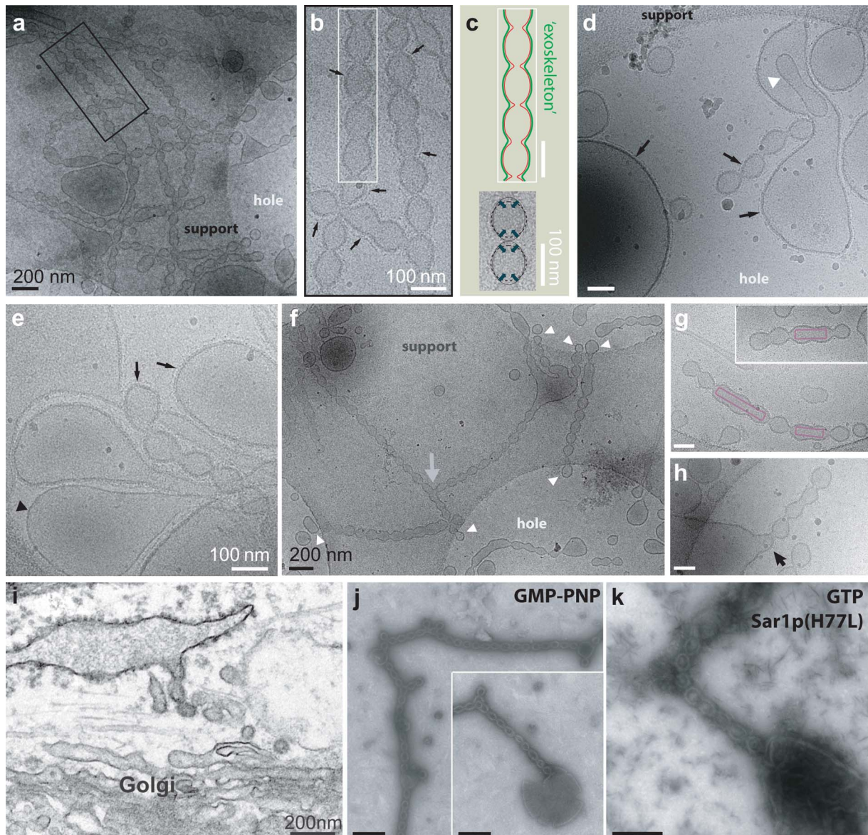
Figure 3 | Generation of multibudded structures by COPII, revealed by EM. Black scale bars = 200 nm; white = 100 nm. (a–h) Cryo-EM view of membrane extensions generated by COPII [ 2\mu\text{M} Sar1p, 320\text{nM} Sec23/24p, 520\text{nM} Sec13/31p, 2.5\text{mM} EDTA, 1\text{mM} GMP-PNP]. (a) Overview and (b) magnified inset. Tubular extensions were coated (arrows in panel b) and carried constrictions at \approx 100 nanometer spacing. (c) Schematic view and model: Drawing of a COPII vesicle string based on cryo-EM. Red denotes the lipid bilayer, green the protein coat. The COPII coat is rigid and may act like an exoskeleton. Bottom: Multibudded vesicles showed elongated shapes. A propensity of the COPII coat to form spheres may contribute to fission at the necks. (d,e) Both large and small vesicles were coated (d,e: arrows), but some large vesicles remained uncoated (e: black arrowhead). An internal vesicle (d: white arrowhead) remained uncoated. (f) Network of multibudded tubules. Occasional branches are seen in (a) and (f) [gray arrow]. Clover-shapes constituted cross-over tubules. Vesicle strings were apparently well-preserved on the carbon support, but often ended at the holes through which the solution had been blotted (white arrowheads). (g) Reconstituted vesicle strings suggest a mechanism for transport of large cargo. Hypothetical cargo is depicted as boxes. A 300\text{ nm} long procollagen bundle, for instance, may occupy three consecutive buds, with fission occurring at the adjoining necks. (h) Some vesicle strings were still connected to a larger liposome and appeared similar to ER exit sites in cells. (i) EM of ER exit sites in a wild type fibroblast cell showed multibudded tubules with a striking resemblance to those produced in vitro from artificial liposomes. (j) Multibudded tubules (including occasional branches) in reconstituted samples were also revealed by negative stain EM. The inset shows a multibudded tubule emanating from a collapsed liposome [ 2\mu\text{M} Sar1p, 320\text{nM} Sec23/24p, 520\text{nM} Sec13/31p, 2.5\text{mM} EDTA, 1\text{mM} GMP-PNP]. (k) The use of the GTP-locked Sar1p(H77L) mutant produced multi-budded tubules in the presence of hydrolysable GTP (negative stain; same sample as in Fig. 2j).
