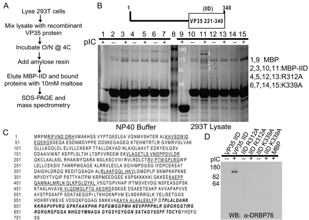
Figure 1. The interferon inhibitory domain (IID) of EBOV VP35 binds to the endogenous double stranded RNA binding protein 76 (DRBP76) in the presence of dsRNA. A , Experimental outline of MBP-VP35-IID pull down. B , Recombinant MBP or MBP fused to wild-type or mutant VP35 IID was incubated overnight with NP40 buffer or 293T cell lysate in the presence (+) or absence (-) of pIC. Unique bands (labeled 1, 2, and 3) were excised and analyzed by mass spectrometry. Results from the protein database search indicated that protein bands 1, 2, and 3 corresponded to RNA Helicase A, nucleolin, and DRBP76 (also known as NFAR-1 and NF90), respectively. C , Primary sequence of the DRBP76 isoform described previously [26]. The underlined regions indicate the enzymatically digested peptides identified by tandem mass spectrometry. The bold-italic region represents the peptide sequence used to generate a DRBP76 specific antibody used in ( D ) that is common to 2 of the 6 isoforms. D , Western blot analysis from the same material used in ( B ) probed with an anti-DRBP76 antibody.
