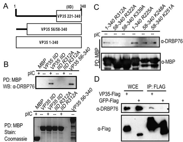
Figure 2. EBOV VP35 amino acids 56–340 bind endogenous DRBP76 in the absence of dsRNA. A , Top panel. Diagram depicting different regions of VP35 IID fused to MBP. B , The VP35-IID constructs were incubated with cell lysate in the presence (+) or absence (–) of pIC. The larger VP35 constructs were only incubated with lysate in the absence of pIC. A fraction of the eluate was analyzed by either coomassie blue stain (bottom) or probed with an anti-DRBP76 antibody (top). C , Characterizing the MBP-VP35 first and central basic patch mutants interaction with DRBP76 in the absence of pIC. The first basic patch mutants used were MBP-VP35 constructs with mutations at amino acids 225, 248, 251. The central basic patch mutants were MBP-VP35 constructs with mutations at amino acids 312, 322, 339. D , A plasmid expressing Flag-VP35 interacts with DRBP76 in 293T cells in the absence of pIC. Western blots against Flag and DRBP76 were performed on IP'd material and on whole cell extracts (WCE)
