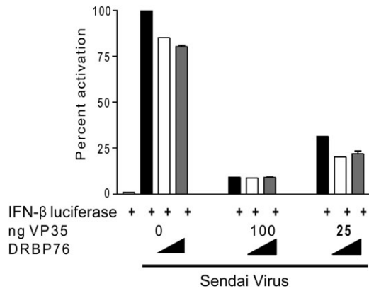
Figure 4. Overexpressed DRBP76 does not alter the ability of VP35 to inhibit IFN-beta reporter activity. An IFN- \beta promoter-firefly luciferase, and a CMV promoter- Renilla luciferase were cotransfected with empty plasmid, a VP35 expression plasmid, or a DRBP76 expression plasmid. The next day, cells were either mock infected or infected with Sendai Virus (SeV) for 18 hours. Cells were lysed and the ratio of firefly luciferase to Renilla luciferase was determined. The positive control (SeV+empty plasmid) was set to 100%.
