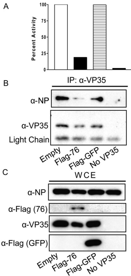
Figure 6. The presence of overexpressed DRBP76 disrupts VP35-NP interaction. A , Graph depicting polymerase activity from the EBOV minigenome co-transfected with empty plasmid, DRBP76-Flag, GFP-Flag or no VP35 (negative control). Each bar represents duplicate samples. B , Fifty percent of the total material from each well in ( A ) was immunoprecipitated with an anti-VP35 antibody and measured by western blot with antibodies to VP35 or NP. C , Western blot of the total cell extract from the same samples as ( B ).
