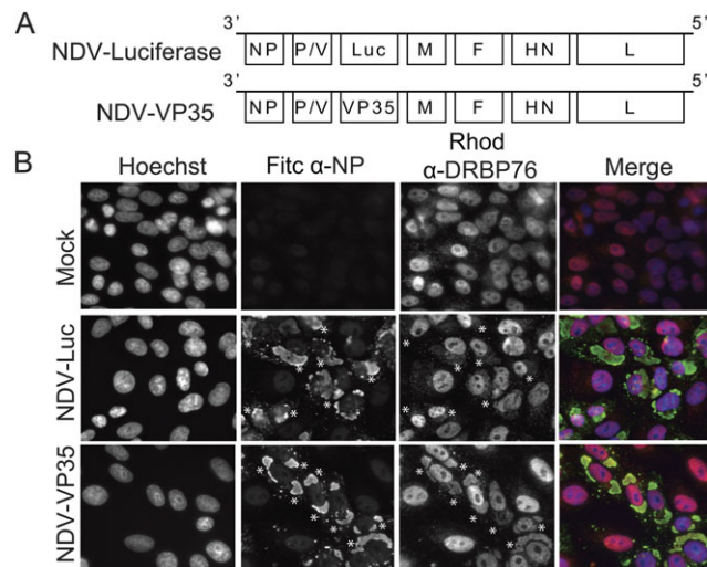
Figure 3. Infection with NDV-VP35 relocates endogenous DRBP76 from the nucleus to the cytoplasm in Vero cells. A , Schematic of the NDV-VP35 and NDV-Luc viruses used in this experiment. B , Vero cells were infected with NDV-Luc or NDV-VP35 at an MOI of 0.5. Twenty-five hours postinfection, cells were fixed and stained for the NP protein (FITC), DRBP76 (rhodamine) and nuclei (Hoechst). DRBP76 relocated to the cytoplasm more dramatically in cells infected with NDV-VP35 compared to NDV-Luc. Stars indicate infected cells/DRBP76 relocation.
