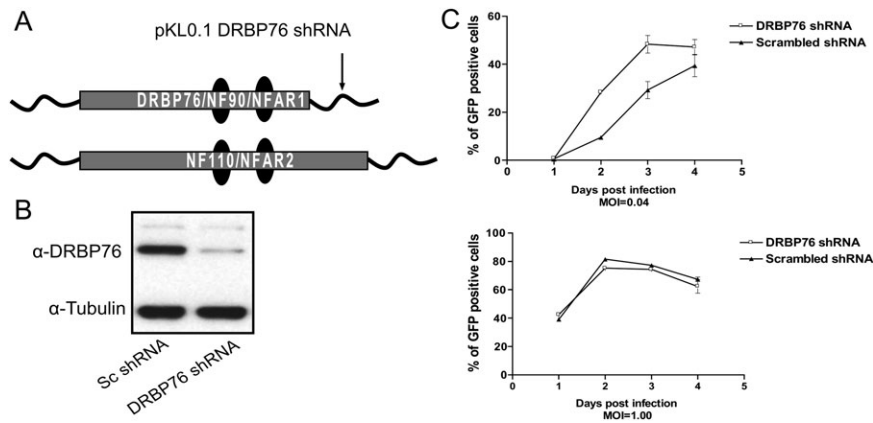
Figure 7. Impact of DRBP76 knockdown in 293T cells on EBOV replication. A , Schematic of DRBP76/NF90 and the related isoform NF110. The location of the sequence targeted by the shRNA is indicated. B , Western blot depicting levels of DRBP76 in both the DRBP76 knockdown and scrambled control cell line. C , Growth of EBOV in the scrambled and DRBP76 knockdown cell lines, measured by the percentage of GFP positive cells.
