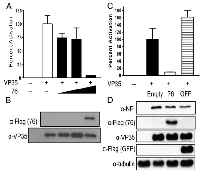
Figure 5. DRBP76 overexpression suppresses EBOV minigenome activity. A , Plasmids encoding T7 polymerase, T7 promoter-expressed EBOV proteins VP30, VP35, NP, L and a model genome with the 3' and 5' noncoding region of EBOV flanking a GFP/CAT reporter were transfected into 293T cells. A firefly luciferase with a CMV promoter was cotransfected as a transfection efficiency control. These plasmids alone, or 10, 50, or 250 ng of CMV driven Flag-DRBP76 were cotransfected with the minigenome constructs. At 44 hours post transfection, cells were lysed and CAT activity was measured and normalized to firefly luciferase activity. Error bars represent the mean and standard error of the mean of triplicate samples. B , Western blot analysis from representative samples from ( A ) to test for expression levels of T7 driven VP35 and CMV driven Flag-DRBP76. C , Similar experiment as in ( A ), but an irrelevant Flag-GFP plasmid at the same concentration as Flag-DRBP76 was transfected (250ng of each). D , Western blot analysis from representative samples from ( C ) to measure protein expression levels of a subset of the transfected plasmids.
