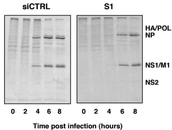
Figure 6. Kinetics of influenza virus protein synthesis in SFPQ/PSF-silenced cells. Cultures of human A549 cells were transfected with SFPQ/PSF-specific siRNA-1 (S1) or control siRNA (siCTRL) as described under Materials and Methods and then infected with VIC virus at a moi of 3 pfu/cell. At the times in hours indicated the cultures were pulse-labelled with 35 S-met-cys and total protein extracts were prepared. The samples were analysed by polyacrylamide gel electrophoresis and autoradiography. The mobility of some of the virus-specific proteins is indicated to the right. doi:10.1371/journal.ppat.1002397.g006
