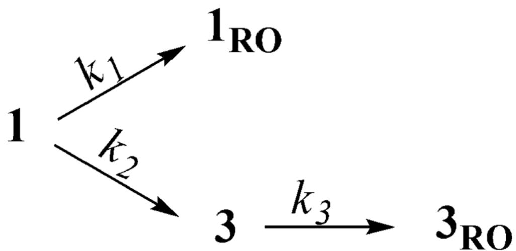
Scheme 3. Simplified kinetics neglecting products that are not measurable during experiment
