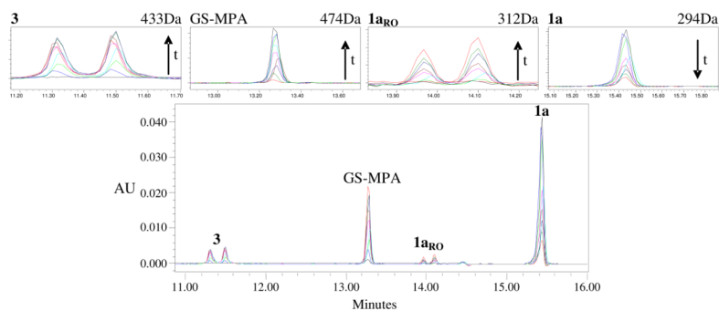
Figure 2. HPLC traces of degradation of 1a in 50mM phosphate buffer with 0.5mM GSSG pH 7.4 @ 37°C over a period of 6days, masses by LC-MS and displayed for (M+H)^+ . The peak area for 1a decreases with time as peak areas for 3 , GS-MPA (mixed disulfide), and 1a RO increase with time, indicating the occurrence of the retro Michael-type reaction. Time arrows indicate the direction of peak area growth or decline with time. Peak 3 consists of two equal peaks representing two diastereomers while the two peaks of 1a RO evolves from ring opening either side of the succinimide with respect to the thioether.
