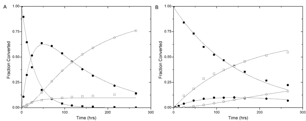
Figure 3. Relative HPLC measured concentrations for 1a (panel A) and 1b (panel B) over time, with constructed curves using derived rate constants and equations 5–8 for (■) 1 (a or b) (□) 1 RO (●) 3 and (○) 3 RO .
