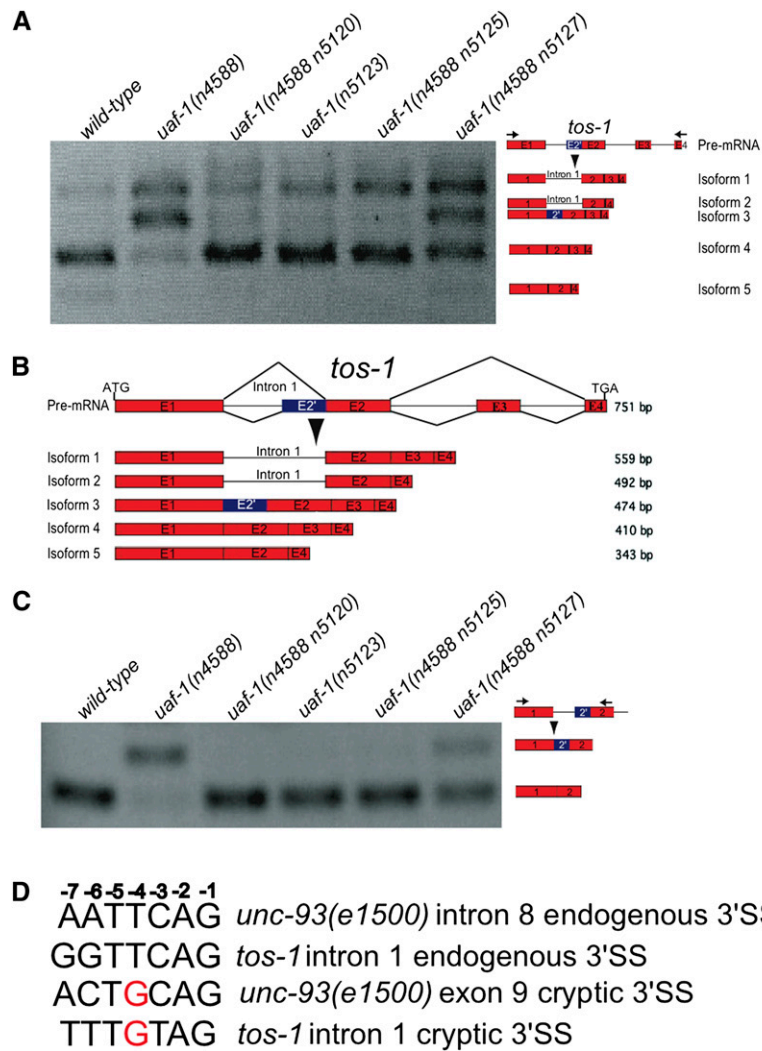
FIGURE 1. uaf-1 mutations alter the splicing pattern of tos-1 . (A) RT-PCR experiments examining tos-1 splice isoforms in different genetic backgrounds. Genotypes are labeled on top. Splice isoforms of tos-1 are illustrated on the right. (Arrows) Positions of PCR primers. (B) Major tos-1 splice isoforms identified by subcloning and sequence determination of RT-PCR products. The base-pair length of each isoform is indicated on the right. (Red boxes) Exons. Splicing at the cryptic 3′ splice site in intron 1 caused an altered exon 2′ (blue). (C) RT-PCR experiments examining the recognition of the cryptic 3′ splice site compared to that of the endogenous 3′ splice site of tos-1 intron 1. Splice isoforms are illustrated on the right. (D) Comparison of the endogenous and cryptic 3′ splice sites from tos-1 intron 1 and unc-93(e1500) intron 8 and exon 9. The position of each nucleotide is labeled on top.
