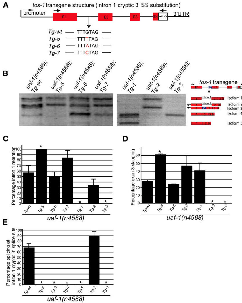
FIGURE 6. 3' splice site substitution and transgenic experiments identified the G nucleotide at position -4 of the intron 1 cryptic 3' splice site as important for recognition by UAF-1(T180I). (A) Illustration of transgene structure and substitutions at the cryptic 3' splice site. (Arrows) PCR primers for detecting transgene-specific transcripts. (B) Splice patterns of the transgenes indicated in a uaf-1(n4588) background as detected by RT-PCR. Splice isoforms are indicated on the right. (C) Quantitative analysis of intron 1 retention of each transgene obtained using the NIH Image J software. (D) Quantitative analysis of exon 3 skipping of each transgene obtained using the NIH image J software. (E) Percentage of the recognition of the intron 1 cryptic 3' splice site of each transgene calculated as the percentage of isoform 3 in the total of isoforms 3, 4, and 5. (*) p < 0.05 .
