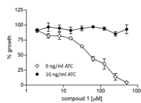
Figure 6. Anti-TB activity of 1 . Mtb bioA-TetON-1 was grown in biotin-free Sauton's medium containing 0 ng/ml or 10 ng/ml ATC and the indicated concentration of compound 1 . Growth was measured as optical density at 580 nm and normalized to growth without 1 . Error bars represent the standard error of the mean of triplicate measurements.
