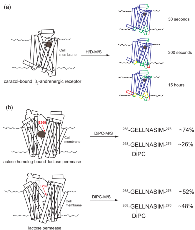
Figure 1. Mass spectrometry in conjunction with hydrogen/deuterium (H/D-MS) exchange and carbodiimide diisopropylcarbodiimide (DiPC-MS) chemical probing reveals membrane protein structural characteristics
