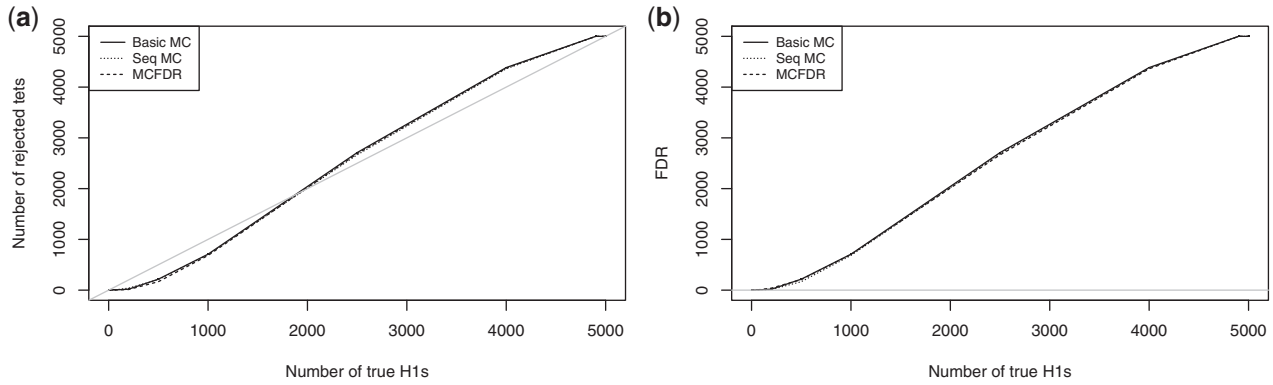
Fig. 2. Behavior of the sequential MC and MCFDR schemes as a function of the number of true H1 . (a) Number of rejected tests as a function of the number of true H1 . (b) Empirical FDR on test collections as a function of the number of true H1 .
