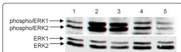
Figure 4 Phosphorylation of ERK1/2 in MO59J spheroids after treatment with 5 Gy irradiation or gefitinib, alone or in combination. ERK1/2 phosphorylation was determined by phospho-ERK immunoblotting using anti-phospho ERK1/2 antibody, and anti-ERK1/2 antibodies against total ERK1/2. Lane 1 - control; lane 2- rhEGF (25 ng/mL); lane 3 - 5 Gy irradiation, lane 4 - gefitinib (50 \mu\text{M} ) and lane 5 - 5 Gy irradiation plus gefitinib (50 \mu\text{M} ).
