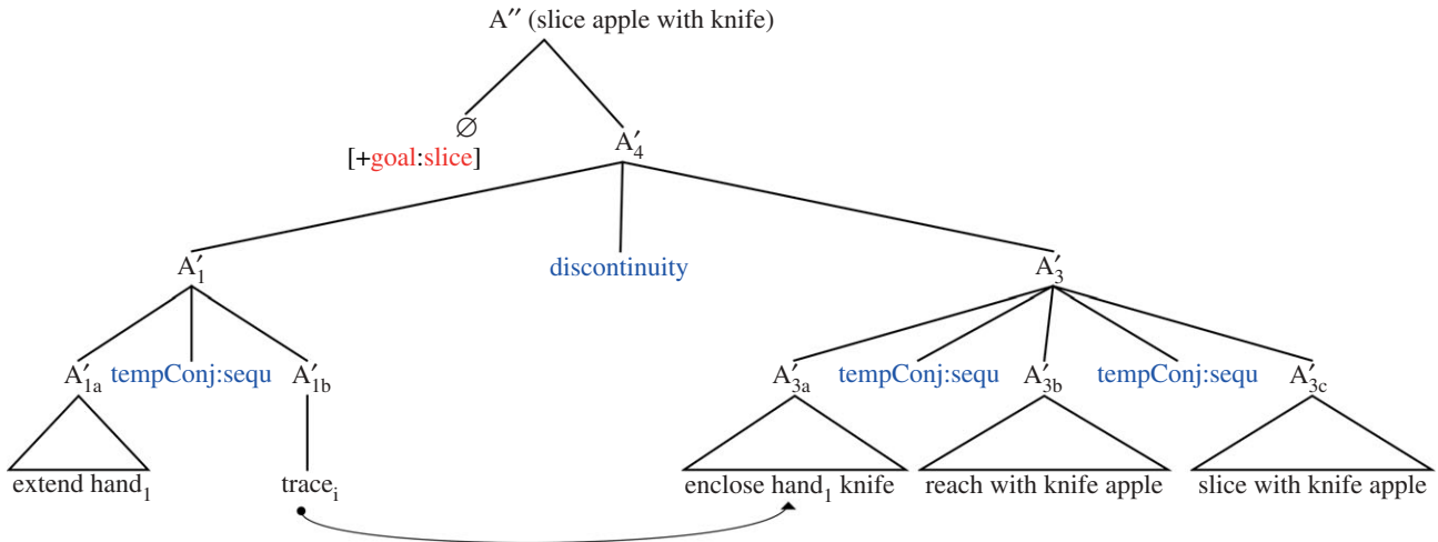
Figure 3. Action parse tree of the structure after applying step 3, i.e. after the move operation has been applied. A'_{3a} shares the same tool complement with A'_{1a} ( hand_1 ) and its object complement (knife) is referred to by A'_{1a} . Therefore, its expected position is semantically exactly after A'_{1a} in position A'_{1b} . However, owing to the disruption by other actions, this position is empty; the action is in position A'_{3a} . Thus, a ‘trace’ of the action is left in position A'_{1b} , which is linked with the action in position A'_{3a} . The two structures A'_1 and A'_3 are not temporally combined, they are discontinuous; the actions that intervene in between may or may not be part of the same action structure. This is what step 4 checks.
