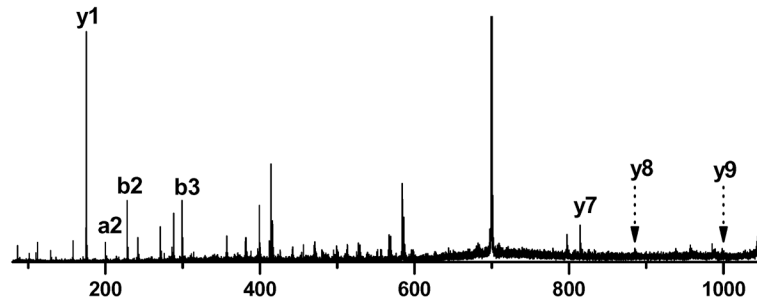
Figure 2. b_2 , b_3 ions and complementary x- and y-type ions in the photodissociation (PD) and postsource decay (PSD) spectrum of NLADLGIQLR.
