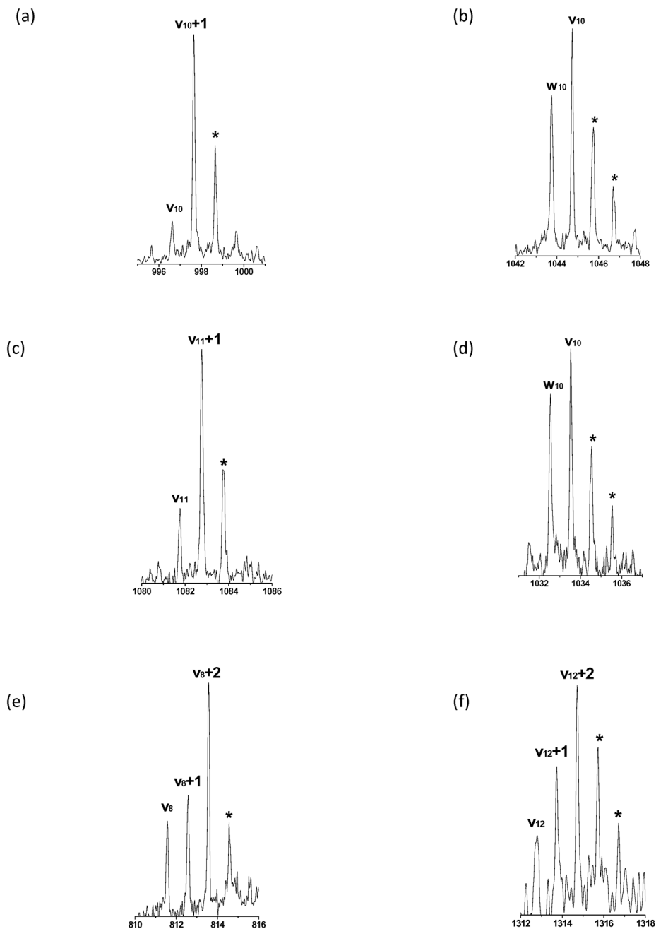
Figure 6. Assignments of (a) v_n+1 radical ion for EGAILSIVLR; (b) v_n , w_n ions of DAIQQAFGAR; (c) v_n+1 radical ion of QLVGQVAANVR; (d) v_n , w_n ions of NGAYLGIQTR; (e) v_n , w_n and v_n+1 radical ions of TVQALGLR; (f) v_n , w_n and v_n+1 radical ions of SLDLDSIIAEVK g . * shows the isotopic peaks and g means that K is guanidinated.
