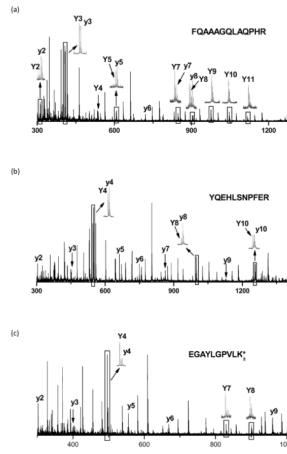
Figure 9. Y-type ions in photodissociation spectra of (a) FQAAAGQLAQPHER; (b) YQEHLSPFER; (c) EGAYLGPVLK g . g means that K is guanidinated.
