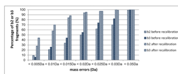
Figure 5. Comparison of the accuracy of identifying b_2 and b_3 fragments before and after recalibration of spectra using y_1 ions.
