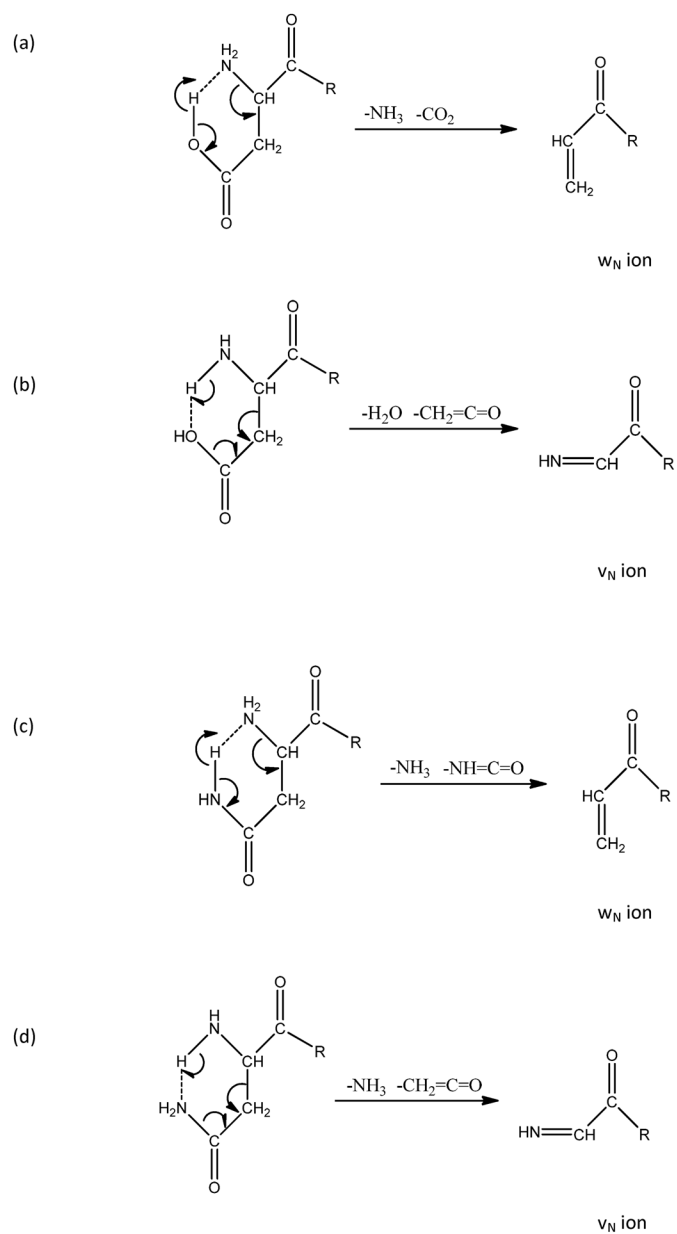
Scheme 2. Pathways to form w_N and v_N from (a)–(b) aspartic acid and (c)–(d) asparagine
