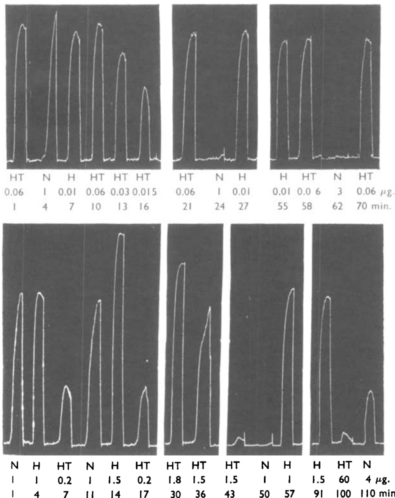
FIG. 1.—Guinea-pig ileum. Contractions due to 5-HT (HT), nicotine (N) and histamine (H). Doses \mu\text{g.} in 2 ml. bath. Above with morphine (1 \mu\text{g.}/\text{ml.} ). Effects on D receptors unchanged by atropine (0.1 \mu\text{g.}/\text{ml.} ) from 18 min. onwards. Dose-ratio=1.3. Below after dibenzylamine (0.1 \mu\text{g.}/\text{ml.} for 30 min.). Effects on M receptors inhibited atropine (0.1 \mu\text{g.}/\text{ml.} ) from 38 min. onwards. Dose-ratio >300 for 5-HT.
