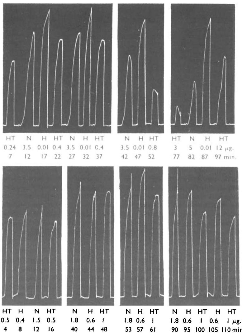
FIG. 2.—Records as Fig. 1. Above with morphine (1 \mu\text{g./ml.} ). Effects on D receptors inhibited by 5-benzyloxygramine (1 \mu\text{g./ml.} ) from 38 min. onwards. Dose-ratio=50 for 5-HT. Below after dibenzylamine (0.1 \mu\text{g./ml.} for 30 min.). Effects on M receptors almost unchanged by 5-benzyloxygramine from 50 min. onwards. Dose-ratio=2.
