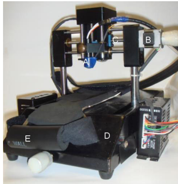
Figure 1 Schematic of the two-axis mechanism. A: Sensor; B: Stepping motor; C: X-axis screw; D: Platform; E: Handgrip.
