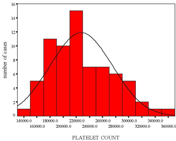
Figure 1 Histogram showing the normal distribution of platelet count.
