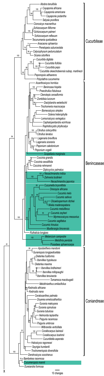
Figure 4 Detail of one of highest global likelihood trees for Cucurbitaceae obtained from combined chloroplast sequences ( matK , rbcl , the trnL intron and spacer, and the rp120-rps12 spacer; 4,966 aligned nucleotides; GTR + G), with parsimony bootstrap values based on 100 replicates shown at branches. Modified from 10, which contains the full tree with all 123 genera. Highlighted are the Cucumis clade and the genera of Cucumerinae in the most recent morphological classification (11).
