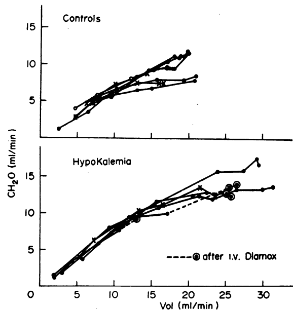
FIGURE 1 Free water excretion in hypokalemia. C H 2 O excretion is plotted as a function of urine volume (= delivery of Na + -containing fluid to Henle's loop). Diamox was used in one study to suppress reabsorption in the proximal tubule.
