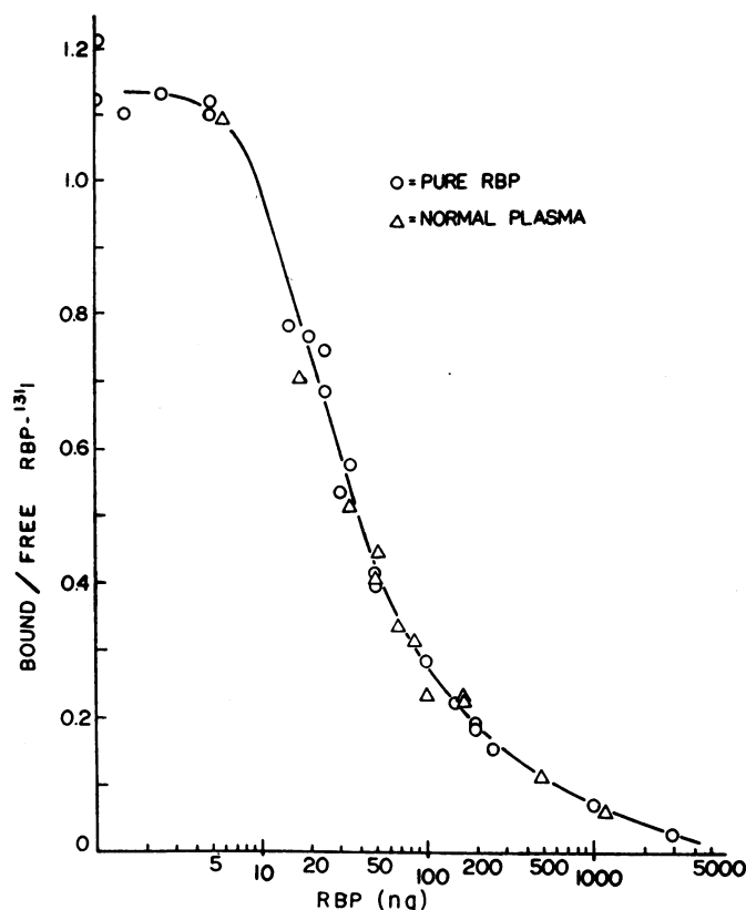
FIGURE 4 The RBP radioimmunoassay standard curve. The figure demonstrates the displacement of RBP- 131 I from antibody by purified RBP and by dilutions of normal plasma. The points for normal plasma were determined by first calculating the mean value for the level of RBP in the sample of plasma from the several assays carried out on that sample. The expected amount of RBP added per assay tube was then calculated from the amount of diluted plasma added. In the figure these values for RBP are plotted against the observed bound/free ratios for the corresponding samples.
