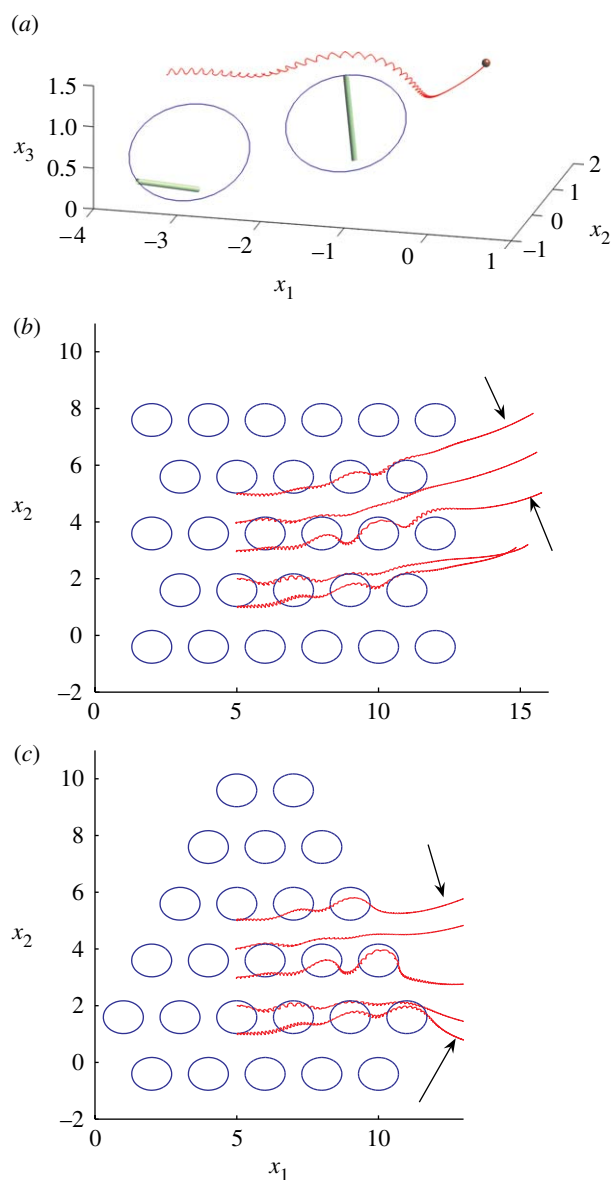
Figure 5. Simulation results obtained with the model and method of Smith et al. (2007). Particle paths are shown due to flow driven by conically rotating cilia beating with tilt angle \theta=35^\circ and semi-cone angle \psi=45^\circ . (a) Advection by two cilia of a particle starting at height 1.2L , where L is cilium length. (b,c) Transport of five particles starting at height 1.2L by approximately rectangular and triangular arrays of cilia (the paths traced by the cilia tips are depicted by ellipses). Note the radial streamlines due to the far-field flow, once the particles leave the array (indicated by arrows).
