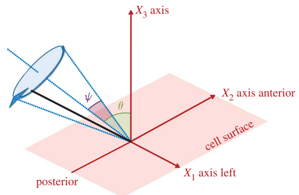
Figure 2. The conical rotation model for an embryonic nodal cilium, with semi-cone angle \psi and posterior tilt \theta . Positive X_1 corresponds to the ‘left’ of the node and negative X_1 to the ‘right’; positive X_2 corresponds to the anterior and negative X_2 to the posterior, as indicated.
