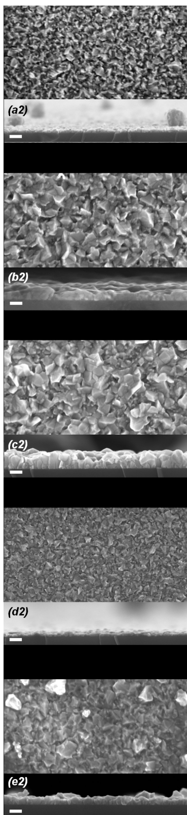
Figure 3 SEM images of ZnO films deposited using different source temperature profiles. (a1-e1) SEMs (top view), (a2-e2)
