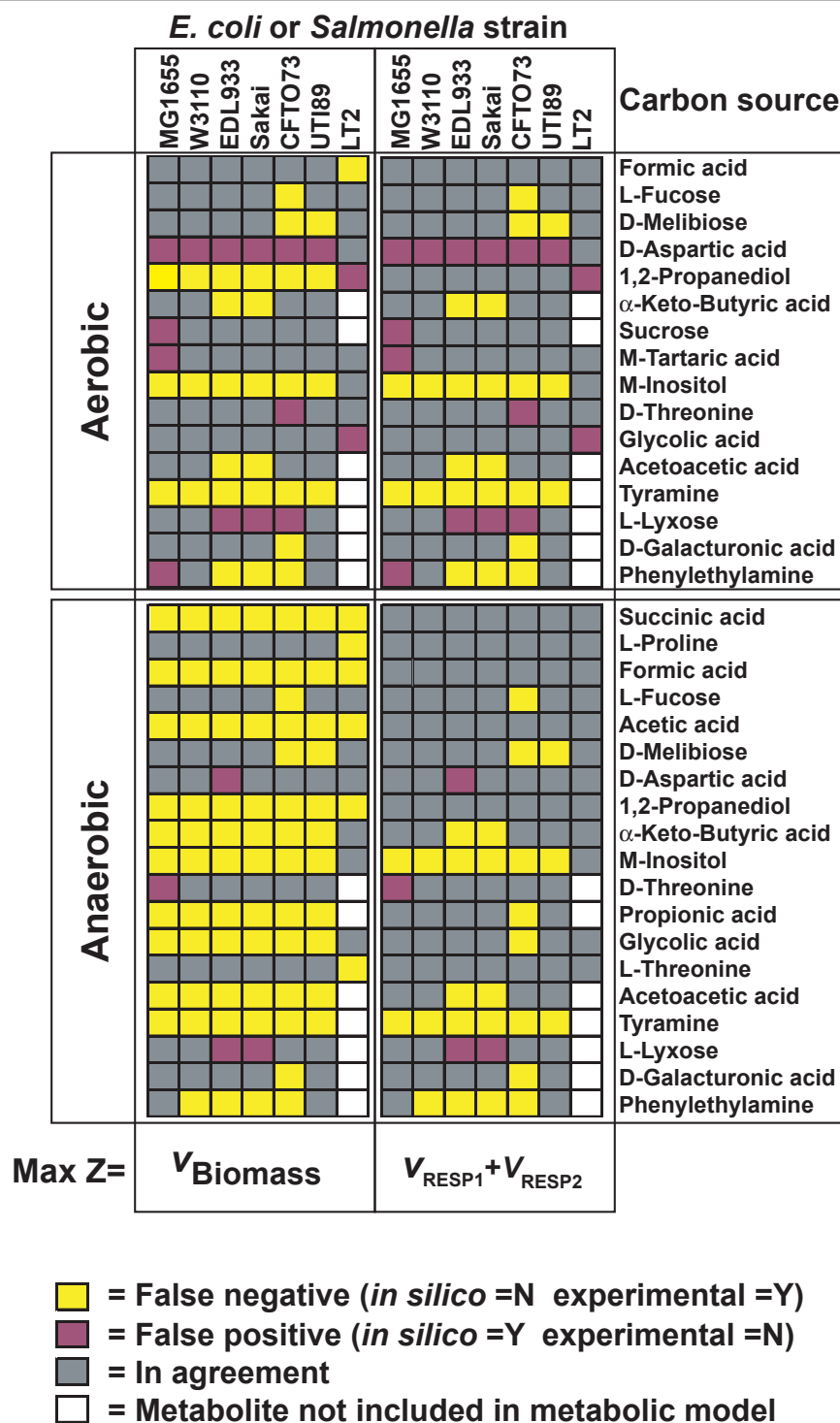
Figure 5 Resolution of in silico and experimental carbon source discrepancies. Carbon source utilization discrepancies for comparison of experimental and in silico data and the respective objective function (Z) used for flux balance analysis.
