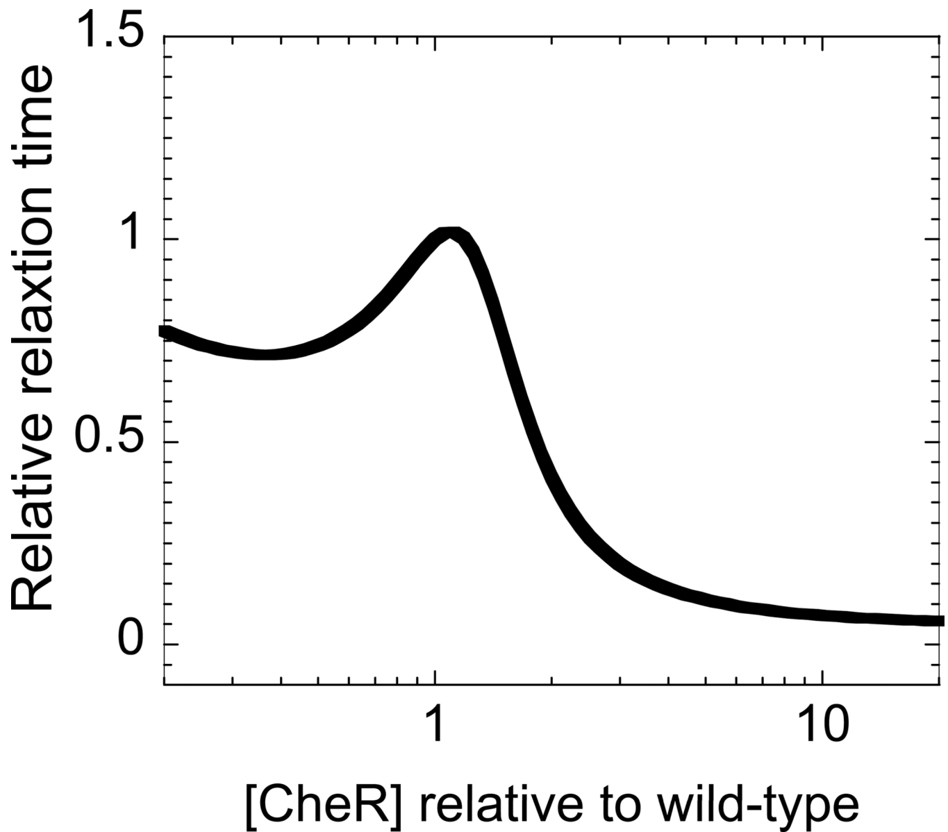
Fig. 2. Relative relaxation time as a function of [CheR]
