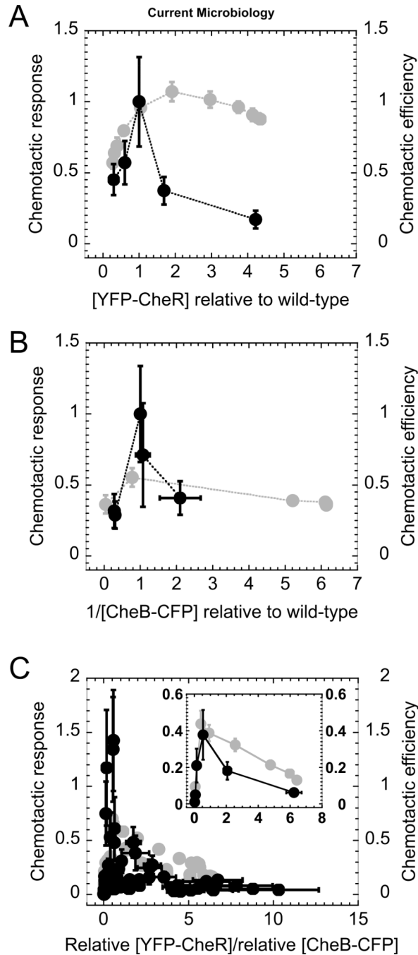
Fig. 3. Effect of relative chemotactic protein concentration on chemotactic behavior
