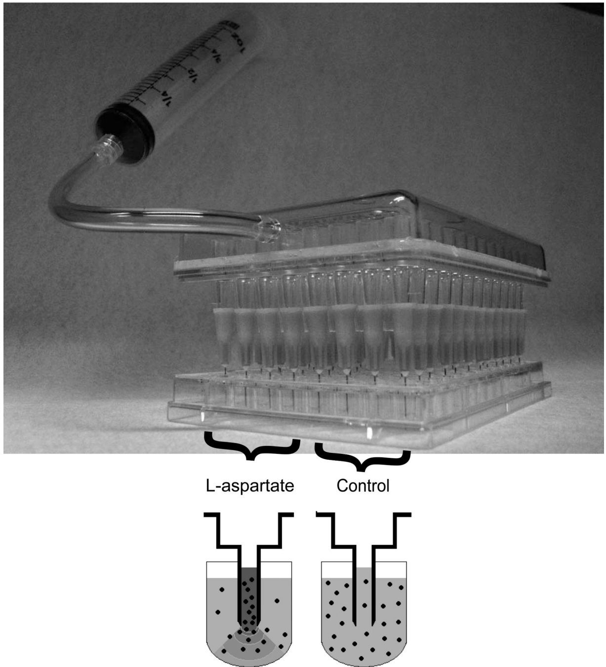
Fig. 1. Schematic of the high-throughput capillary apparatus
