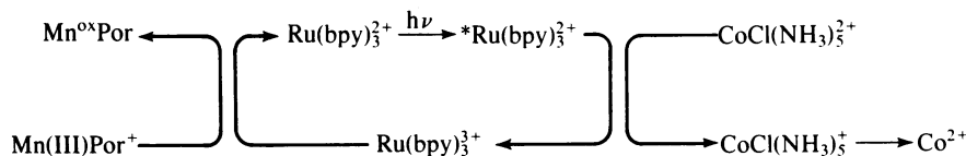
FIG. 1. Schematic diagram of the arrangement used in the photoinduced oxidation of Mn(III)Por + in homogeneous solution. Ru(bpy) 3 2+ is the photosensitizer and CoCl(NH 3 ) 5 2+ is the electron acceptor.
