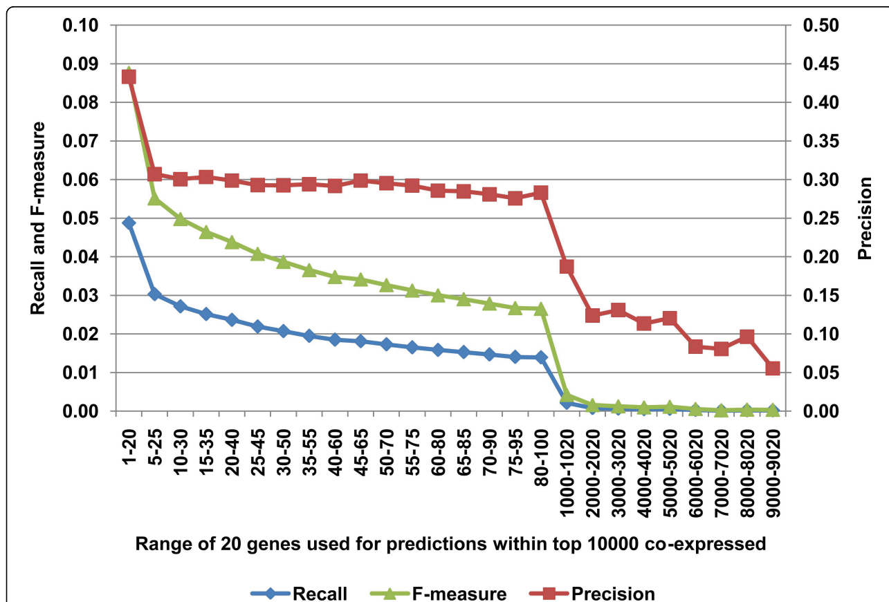
Figure 3 Influence of top co-expressed gene selection on prediction power. Only top co-expressed genes achieved best balance of recall and precision (F-measure), which dropped dramatically as less well co-expressed genes were selected.
