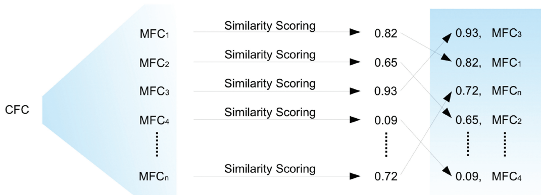
Figure 1. If an miRNA is involved in a specific cancer, the miRNA target genes and the cancer-related genes would be associated with the same or similar functions. The FCS can be used to quantify the association between miRNAs and a specific cancer. In the first step (STEP 1), cancer-related genes are obtained from several cancer databases or experimental results. Next, functional enrichment analyses based on GO are performed on a CFC and an MFC, and the significantly enriched functional categories of the CFC and MFC are obtained. In the second step (STEP 2), for the i th miRNA, an FCS is calculated between MFC_i and CFC using a semantic similarity measurement. FCSs can be determined for all the candidate miRNAs. Higher FCS values reflect a closer relationship with the cancer.
