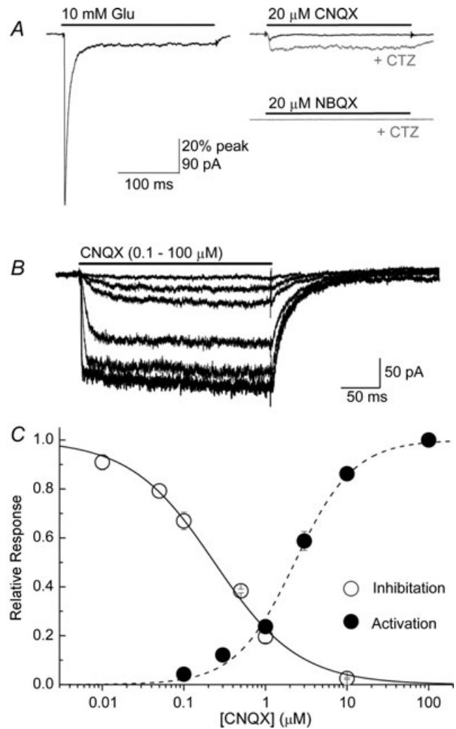
Figure 3. Activation or desensitization by CNQX contributes little to high-affinity AMPAR block A, left, response from a patch containing GluA1 and stargazin to 10 mM L-Glu (patch no. 080201p1). A, right, responses from the same patch to 20 μM CNQX (upper) or 20 μM NBQX (lower) either alone (black) or in the continual presence of 100 μM CTZ (grey). B, responses from GluA1 with stargazin to varying concentrations of CNQX in the presence of CTZ and with 400 mM NaCl (patch no. 110216p1). C, summary of inhibition curve for GluA1 plus stargazin from Fig. 2 and activation curve for CNQX in the continual presence of CTZ.
