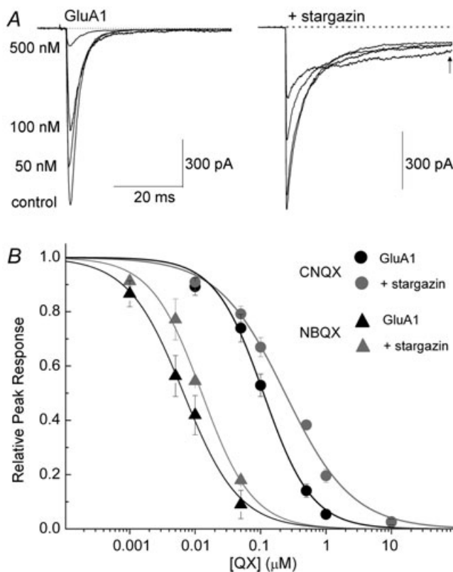
Figure 2. Stargazin does not substantially alter the blocking ability of CNQX or NBQX A, inhibitory effect of CNQX on responses evoked by 10 mM L-Glu on patches of GluA1 alone (patch no. 070827p1) or with GluA1 and stargazin (patch no. 070817p1). B, inhibition plots of block by CNQX (circles, n = 4-17 ) and NBQX (triangles, n = 3-10 ) of peak L-Glu responses evoked from patches containing GluA1 alone (black) or with stargazin (grey).
