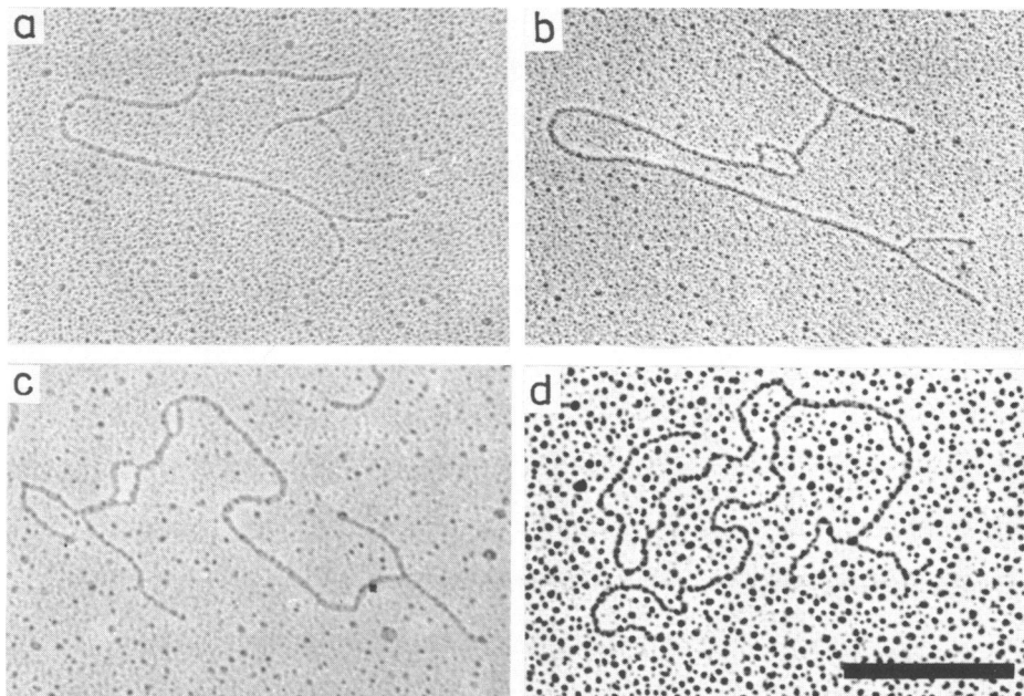
FIGURE 2. Micrographs of partly denatured ColE1 DNA molecules fixed at 69.3°C (a), 71°C (b), 72.2°C (c), 74.7°C (d). Arrows show the denatured regions. The bar represents 0.4 \mu m.
