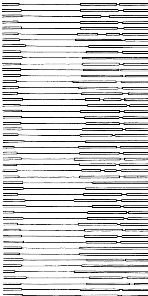
FIGURE 3. The set of molecules used for constructing the denaturation map corresponding to T_p=74.7^{\circ}\text{C} .
