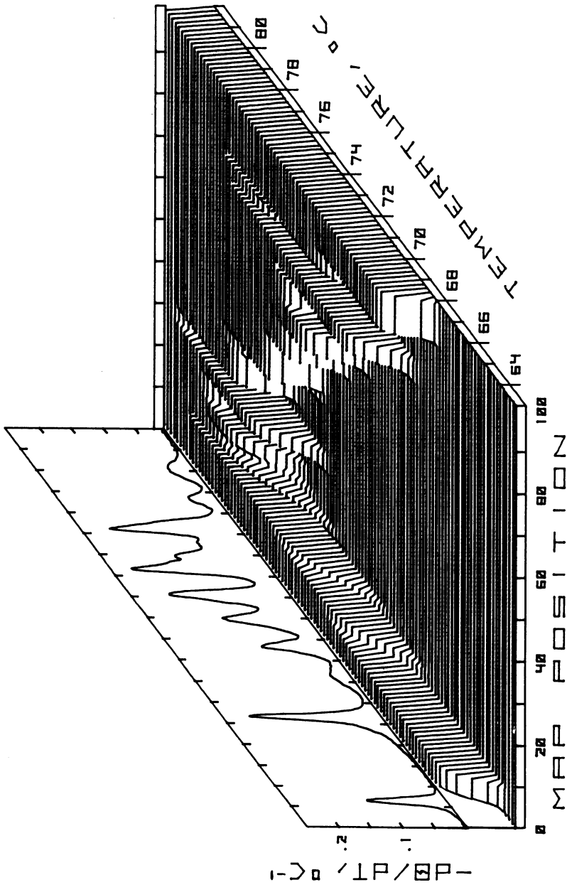
FIGURE 8. The three-dimensional diagram illustrating the process of the heat melting of ColE1 DNA. The Z co-ordinate represents the probability of the melting of a given region of the molecule at different temperatures. For comparison the differential melting curve is shown on the left.
