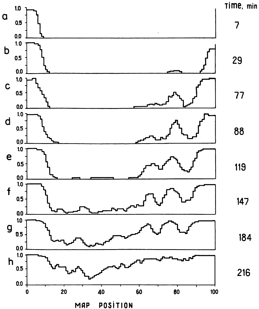
FIGURE 6. Formaldehyde denaturation maps corresponding to different times after the onset of the unwinding reaction. The times are shown on the right.
