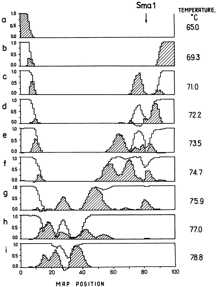
FIGURE 4. Denaturation maps of ColeE1 DNA corresponding to different melting stages. The shaded area in each map is the difference obtained by subtracting from this map the map for the preceding temperature of fixation. The temperatures, T_f , are shown on the right. The arrow indicates the cleavage site for Sma1 endonuclease.
