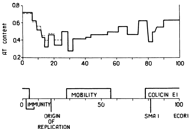
FIGURE 5. The distribution of AT-pairs over the ColE1 DNA molecule. (solid line) Dashed line represents the average AT content of the appropriate regions of pA02 DNA /23/ (see text). Shown below is a functional map of the plasmid ColE1 /18/.
