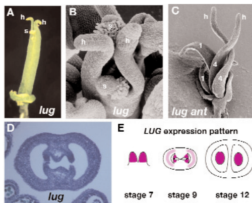
Figure 24. LEUNIG is involved in fusion of the carpels. (A) lug fruit, showing horn like protrusions of the valves (h) above the stigma (s). (B) Close up of the unfused apex of a lug gynoeceium. There are two medial stigmatic surfaces (s) and two later horn shaped protrusions from the valves (h). (C) lug ant double mutant showing the two completely unfused horn shaped carpels of the fourth whorl (4). Because of the homeotic affects of lug on the other floral organs, the medial first whorl sepals have also been converted to horn shaped unfused carpels (1). (D) Cross-section of a lug gynoeceium with two carpels at stage 10 showing the failure of the septum to fuse. (E) LUG is expressed throughout the carpels at stage 7. Carpel expression is reduced in stage 9, but strong LUG expression is detected in the developing ovule primordia. At stage 12 LUG expression is restricted to the ovules. A-D: from Liu et al., 2000.
