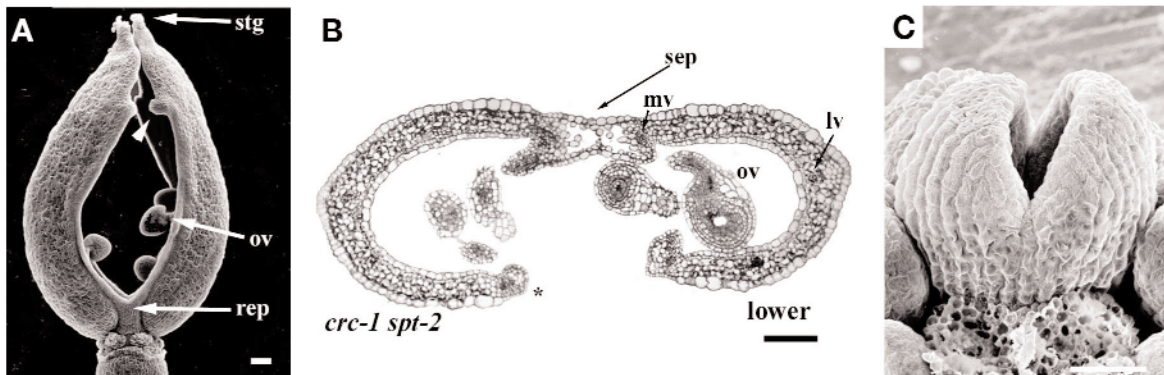
Figure 30. The crc spt double mutant. (A) SEM of a crc spt double-mutant fruit showing that the carpels are largely unfused. The stigma (stg), ovules (ov) and replum (rep) are labeled. (B) Cross-section of a crc spt gynoecium of the lower part of a mature flower. The septum (sep), medial vascular bundle (mv), lateral vascular bundle (lv), and ovule (ov) are labeled. (C) SEM of a crc spt gynoecium at stage 8, showing that the carpels are largely unfused and curve inward. Scale bars in A-B represent 100 \mu m and the scale bar in C represents 25 \mu m. A-C: from Alvarez and Smyth 2002.
