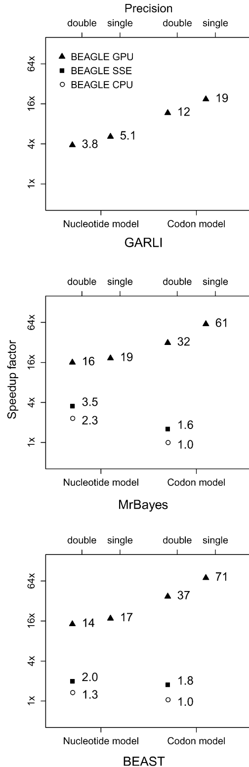
FIGURE 1. Performance using the BEAGLE library relative to the native sequential CPU implementations of phylogenetic analysis programs GARLI, MrBayes, and BEAST. Speedup factors are on a log scale.
