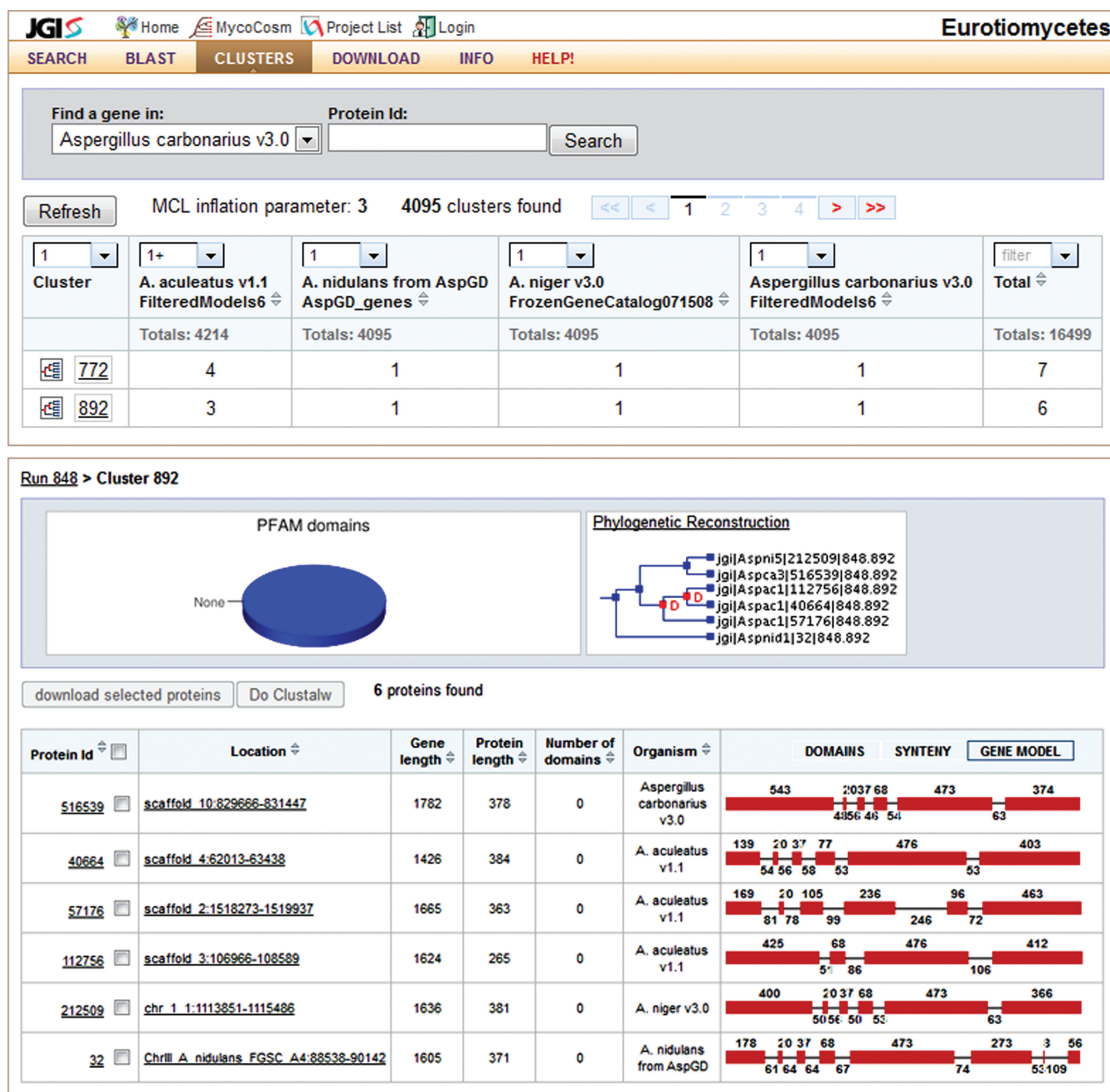
Figure 4. MycoCosm comparative view includes several functions designed for analyzing groups of genomes (listed in the top menu) as illustrated by Cluster view. The Cluster front page (on top) lists two largest clusters of genes conserved in all four Eurotiomycetes and expanded in Aspergillus aculeatus , after using filters (1+:1:1:1). Cluster details page (on bottom) shows six members of the cluster 892, their intron–exon gene structures (right column), PFAM domain composition (pie chart in the middle, no predicted domains here) and species-reconciliated gene tree suggesting two gene duplications Aspergillus carbonarius (red nodes D on the tree in the middle).
