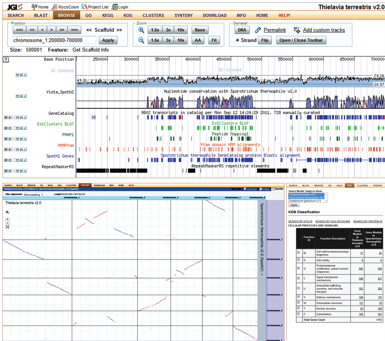
Figure 3. Genome-centric view of the MycoCosm includes several tools (listed in the top menu) and illustrated here by Genome Browser (on top), Synteny by interactive VISTADot plot (lower left) and KOG functional profile (lower right). Genome Browser tracks shown for a thermophile Thielavia terrestris (14) include GC content (light blue), VISTA-based genome conservation (blue and red curve), automatically predicted (blue) and manually curated (red) gene models, transcriptomics (light green) and proteomics (dark green) data, PFAM domains (orange), BLASTx hits against proteins of related organism (blue), and repeats (black). Dot plot is based on VISTA whole genome alignments of two genomes and interactively displays syntenic blocks (collinear in blue or anti-sense in red). KOG profile summarizes functional annotations of genes according to this classification and allows comparison of gene counts in each category between related genomes (last two columns).
