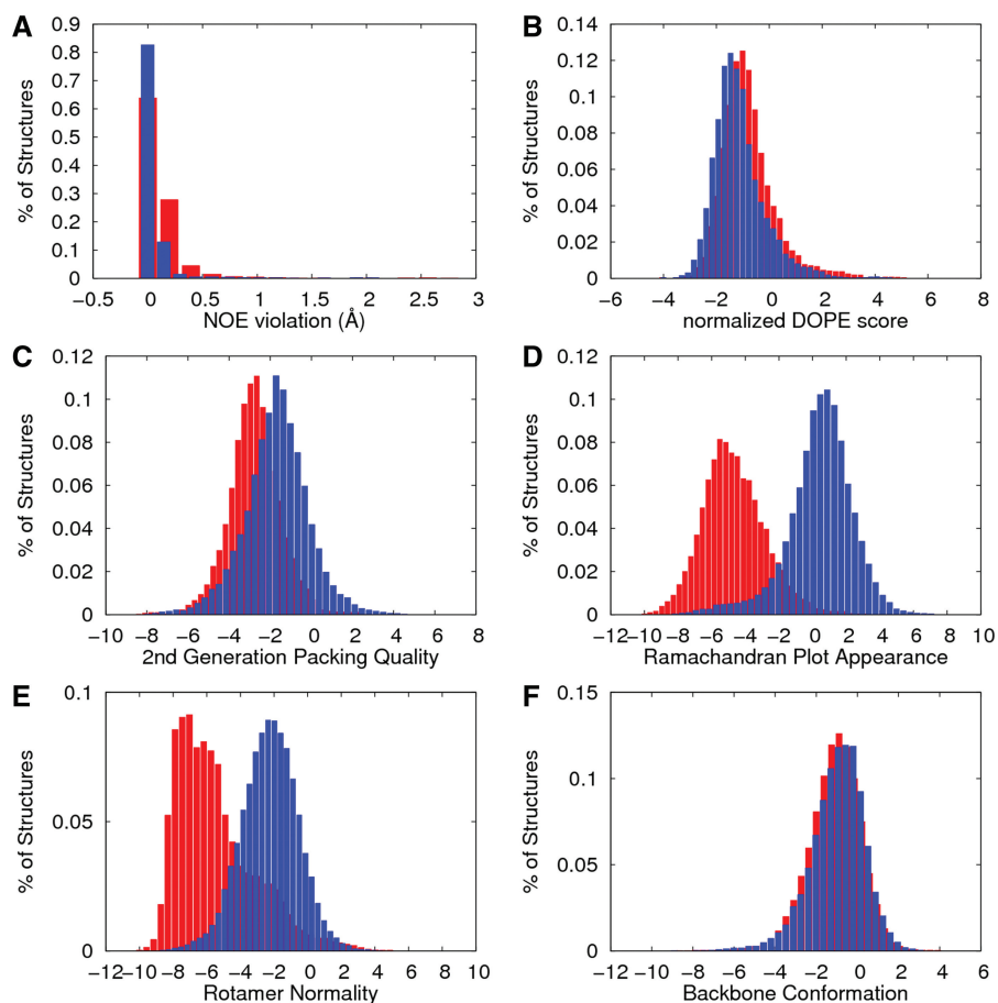
Figure 1. Distribution of the protein quality assessment of the original (red) and refined structures (blue bars). The figures present the distributions of the 2405 selected NMR structures as follows: (A) the RMS value of the NOE violations, (B) the normalized DOPE score, (C) the 2nd-generation packing quality (all backbone and side chain contacts), (D) the Ramachandran plot appearances, (E) the \chi_1 - \chi_2 rotamer normality and (F) the backbone conformation. The values were measured by dDFIRE, AQUA and WHAT_CHECK.
