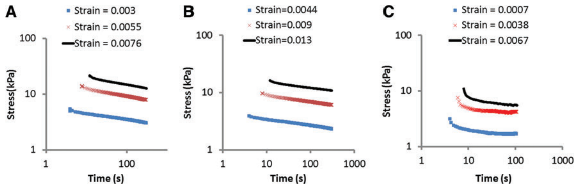
FIG. 9. Stress relaxation as a function of initial strain for animal-matched (A) ACL and (B) BLB explant in adult sheep and (C) adult patellar tendon. Color images available online at www.liebertonline.com/tea
